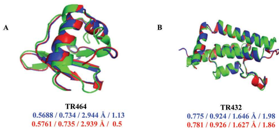
Fig. 2. Structural superposition of initial model (blue) and refined model using 3Drefine (red) on the native structure (green) for two CASP8 Targets. The values under each model indicate GDT-HA, TM-score, RMSD and MolProbity score respectively before (blue) and after (red) refinement.
