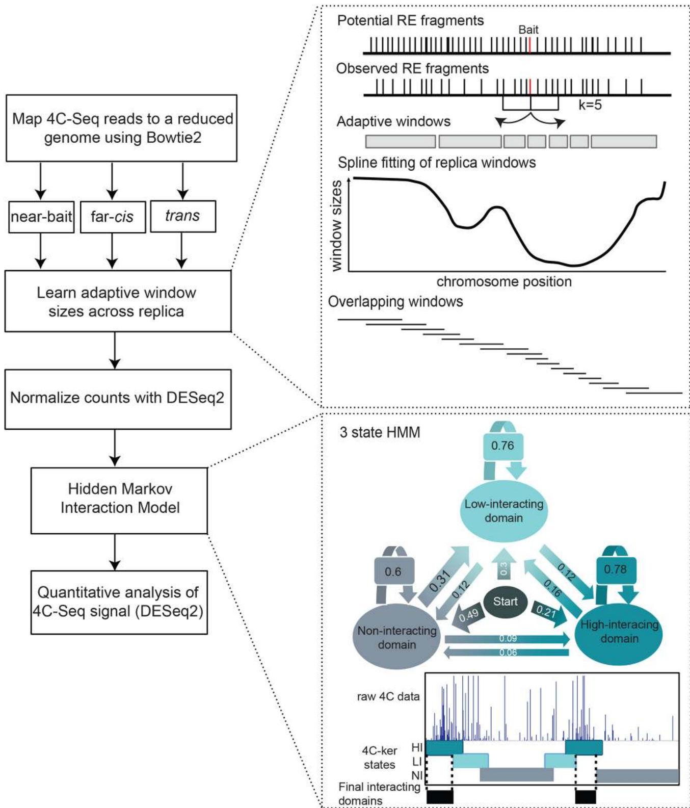
Fig 1. Workflow of 4C-ker. The key features of the method are outlined in the figure. A more detailed explanation of each section can be found in the materials and methods section.
