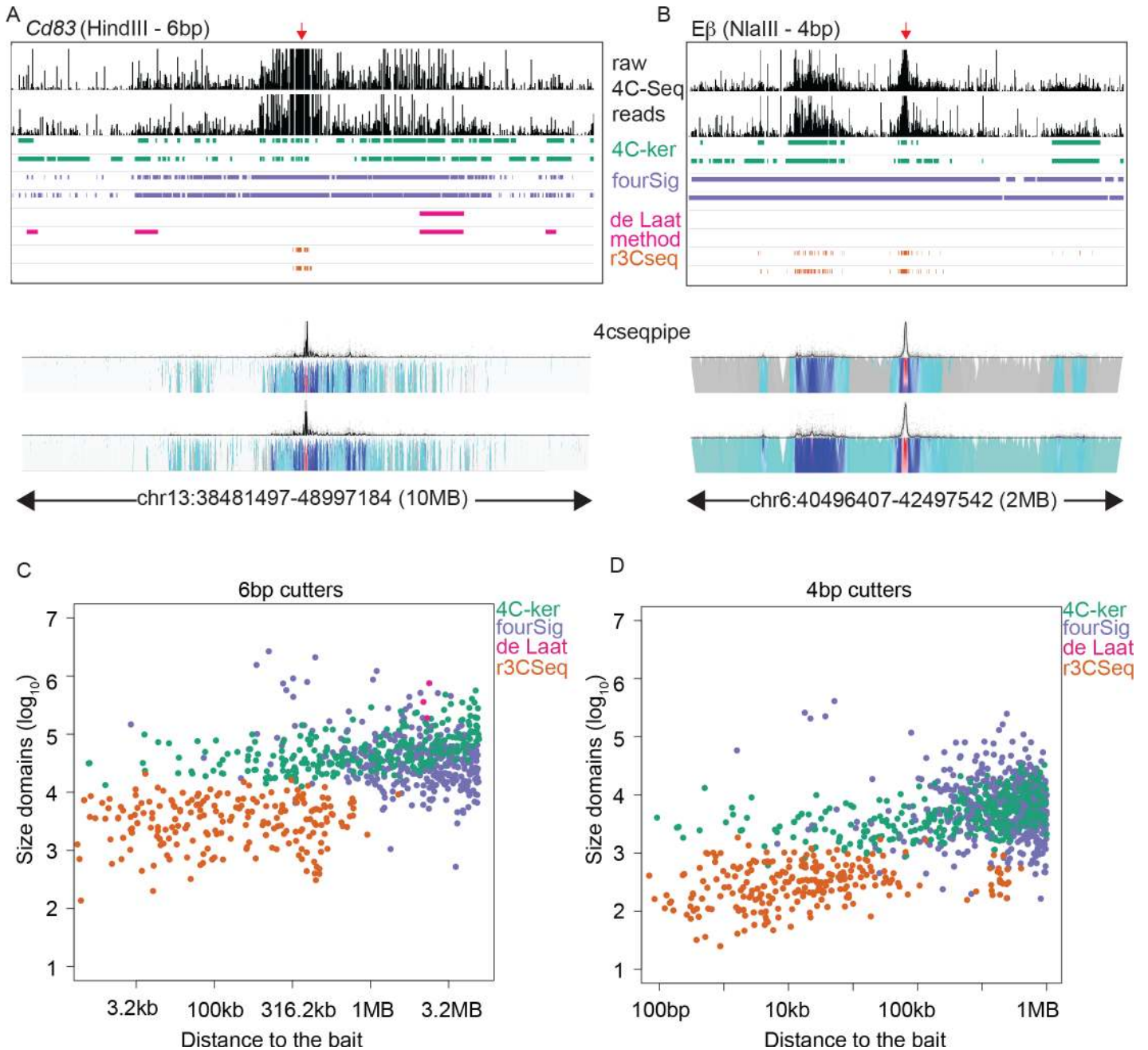
Fig 2. 4C-ker outperforms other methods in the region near the bait when the similarity of interacting regions between replicates is examined for four methods. (A-B) Example datasets for 6bp and 4bp cutter experiments. Raw 4C-Seq reads are shown for a 10MB region around the bait in (A) and 2 MB in (B). Experiment in A was performed using activated B cells digested with HindIII and a bait near the Cd83 locus. Experiment in B was performed in double negative T cells digested with NlaIII and a bait near the Eβ enhancer of Tcrb . Significant interactions determined by each method for 2 replicates are shown below the raw 4C-Seq profile. Domainograms generated using 4cseqpipe are displayed for the same region. (C-D) Each dot represents the distance of the midpoint of each interacting domain to the bait plotted against its size. Plots only contain domains that overlap by 50% between replicates.
