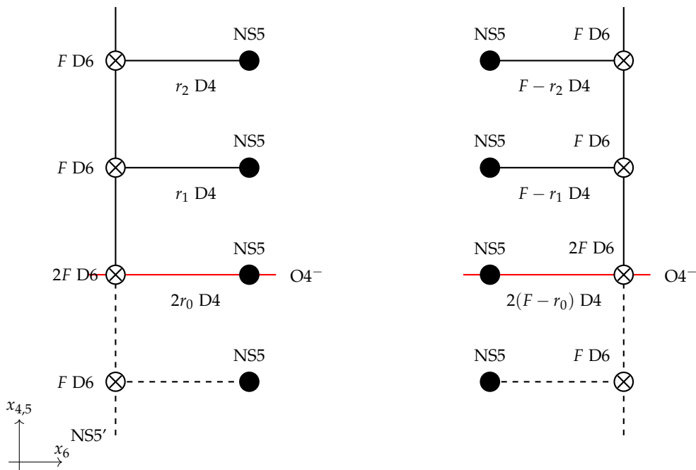
Figure 9. Electric and magnetic sides of the duality for \text{Sp}(2N) gauge theories with adjoint matter.
