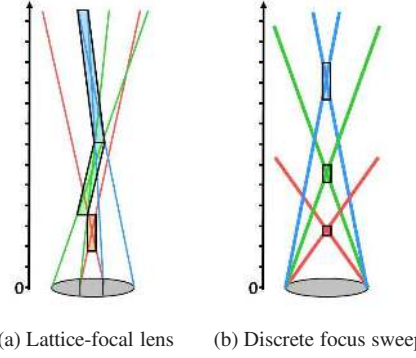
Figure 8: Focus sweep vs. the lattice-focal lens. (a) Lattice-focal lens whose aperture is divided into 3 differently-focused bins. (b) Discrete focus sweep, dividing the integration time into 3 bins, each focusing on a different depth (note that an actual focus sweep camera varies focus continuously). Depth ranges with defocus diameter below a threshold are colored. While in both cases each bin lets in 1/3 of the energy, the sub-apertures for the lattice-focal lens are narrower than the full aperture used by the focus sweep, hence the effective DOF for each of the lattice-focal bins is larger.
