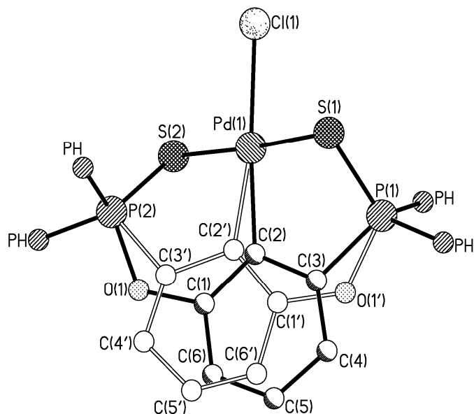
Figure 1S. Schematic view of complex 4c with the central fragment shown as a superposition of two isomers in 70 to 30 ratio. The minor component is indicated by open lines.
