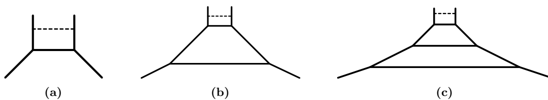
Figure 5. Webs for SU(N)_N with N = 1, 2 and 3 .
