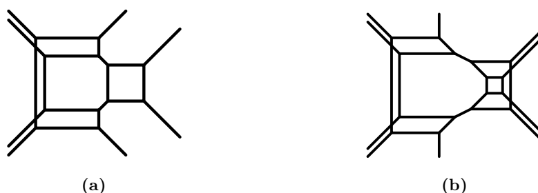
Figure 11. 5-brane webs for (a) \text{Sp}(2) \times \text{SU}(2) quiver, (b) \text{Sp}(2) \times \text{Sp}(2) quiver.
