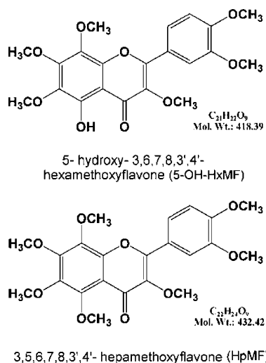
Figure 1. Chemical structures of "5-OH-HxMF and "HpMF.
