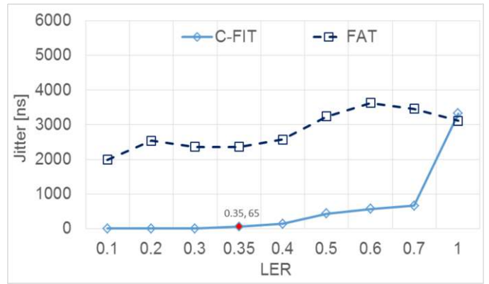
Figure 11: Jitter vs. Load to Ethernet Ratio for number of flows 1 to 3 and line rates 1 to 9.
