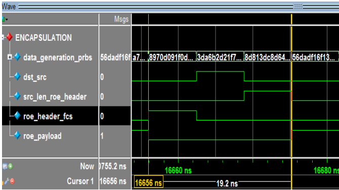
Figure 5: FPGA pre-synthesis simulation of CoE encapsulation.
