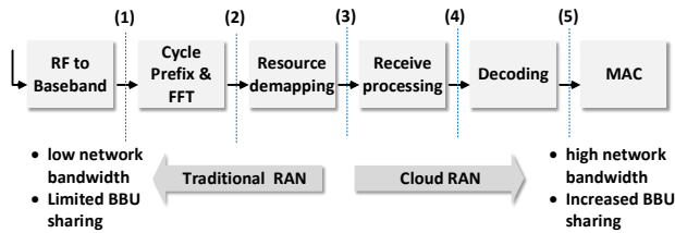
Fig. 2 Functional split of BS processing [6],[11],[21]
