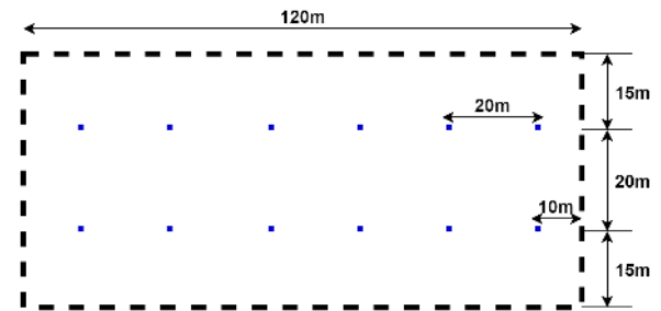
FIGURE 9. Indoor Hotspot site Layout.
