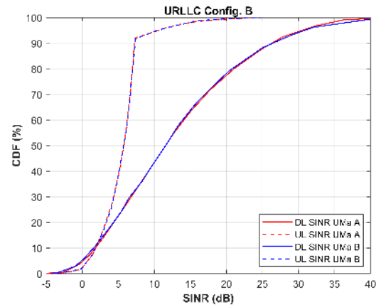
FIGURE 27. URLLC configuration B SINR distribution .
