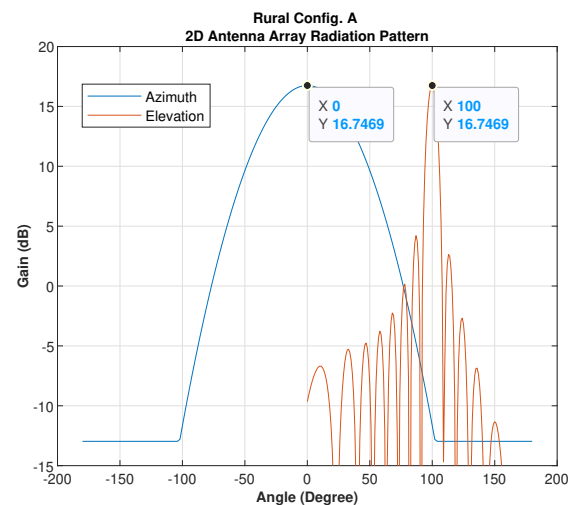
FIGURE 4. 2D Antenna array radiation pattern for rural eMBS config. A.
