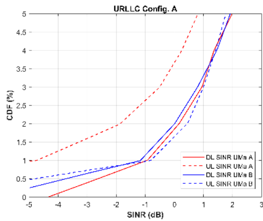
FIGURE 25. 5 th percentile SINR distribution for URLLC configuration A.
