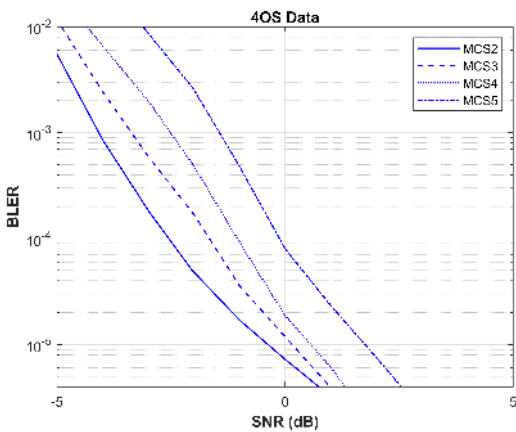
FIGURE 30. LDPC BLER 4 OS-Data for QPSK (1st attempt) .
