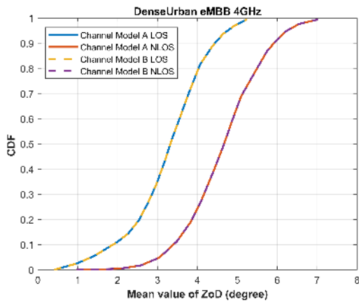
FIGURE 18. Dense Urban (4 GHz) ZoD (degree) Mean value.
