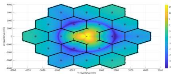
FIGURE 6. Antenna Sector plot for RMA Configuration A.
