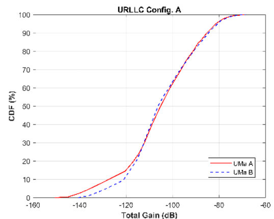
FIGURE 23. URLLC configuration A Total gain.
