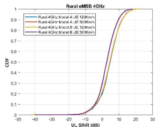
FIGURE 20. Rural-eMBB (4 GHz) UL SINR distribution test environment.
