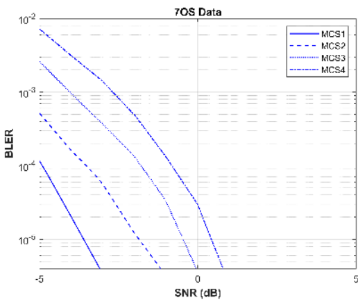
FIGURE 31. LDPC BLER 7 OS-Data for QPSK (1st attempt).
