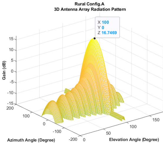
FIGURE 5. Antenna Array Radiation Pattern for 8x1 elements with Scan angle= 0° and Etilt angle = 100°.
