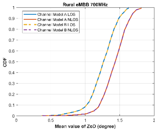
FIGURE 17. Rural (700 MHz) ZoD (degree) Mean value.
