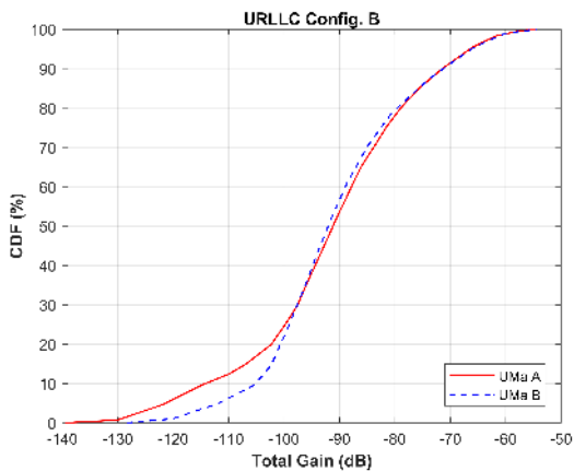
FIGURE 26. URLLC configuration B Total gain.
