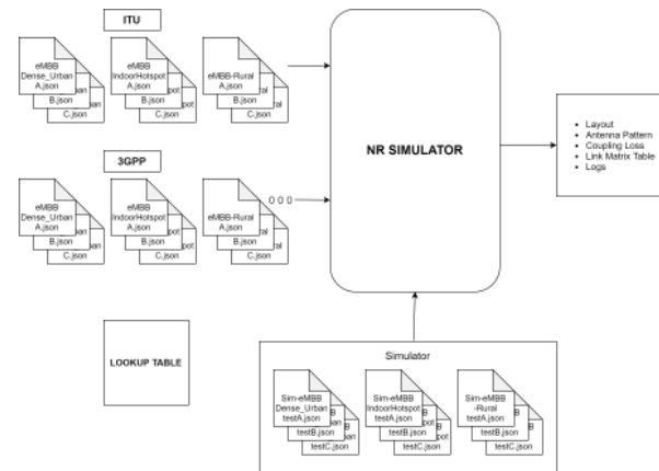
FIGURE 3. 5G New Radio Simulator Setup.
