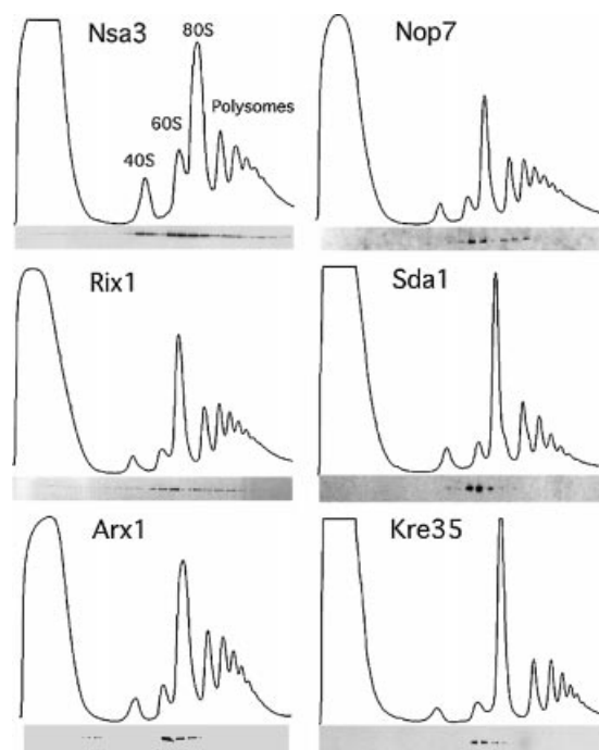
Fig. 1. Reverse-tagged protein baits of the Nug1-containing 60S pre-ribosome are associated with pre-ribosomal particles of different sizes. The sedimentation behavior of the indicated TAP-tagged proteins was analyzed on sucrose density gradients, and ribosomal fractions (40S, 60S, 80S and polysomes) were determined by OD 254 measurement of the gradient fractions (upper graph). Western blot analysis of these gradient fractions using anti-ProtA antibodies reveals the position of the indicated TAP-tagged baits (lower panel). Note that some baits (e.g. Nsa3) exhibit a broad distribution on the sucrose gradient, whereas other baits (e.g. Kre35) exhibit a distinct peak at ~60S (see text).
