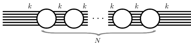
Figure 3. Type IIA description of the system of N M5-branes probing the \mathbb{C}^2/\mathbb{Z}_k singularity: here we are drawing schematically the X^6 direction for the tensor branch. One obtains N NS5-branes sitting on top of k infinite D6 branes.
