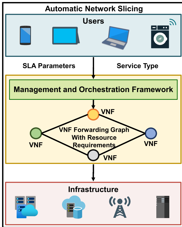
FIGURE 6. Automated network slicing framework.
