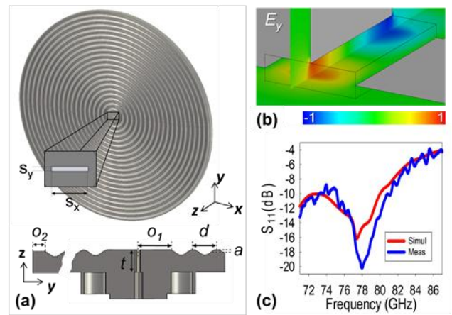
Fig. 1. Sinusoidal Bull's Eye antenna (a). Detail of the slot resonance (b). Measured (blue curve) and simulated (red curve) S_{11} (c).
