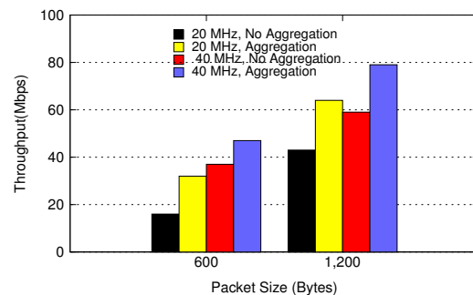
Figure 3: Average throughput achieved on a isolated 802.11n link under different combinations of channel width and aggregation mechanisms.
