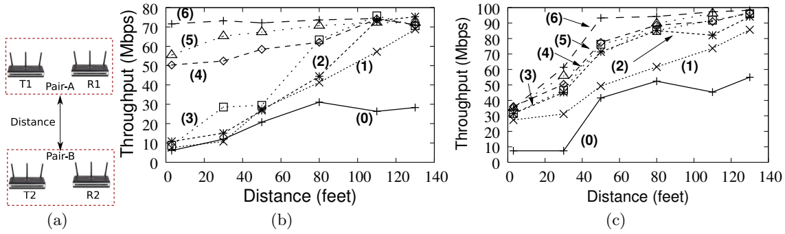
Figure 5: (a) Setup used for channel overlap experiments. The transmitter and the receiver are co-located while the separation (distance and channel) between the pairs is increased for each run. (b) UDP throughputs for a channel bandwidth of 20 MHz. (c) UDP throughputs for a channel bandwidth of 40 MHz.
