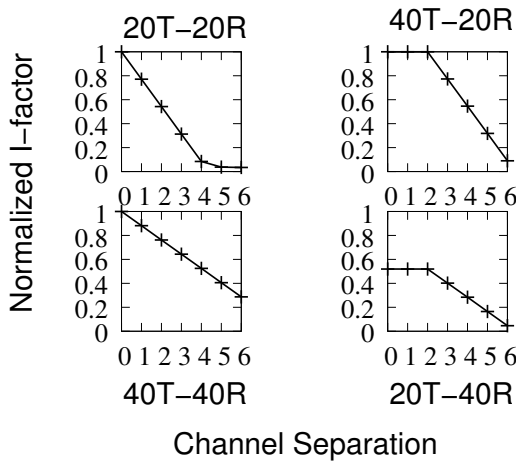
Figure 6: Theoretical I-factors for various interferer and receiver combinations.
