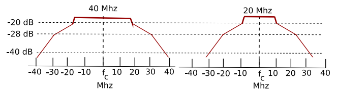
Figure 7: Transmit spectrum masks for 40 MHz and 20 MHz channels for the physical layer in IEEE 802.11n standard
