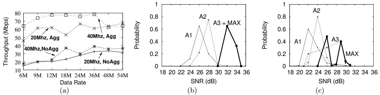
Figure 4: (a) Throughput of an 802.11n link severely degrades in presence of an 802.11g link operating on a lower data rate. Frame aggregation improves the throughput of the 802.11n link by providing temporal fairness .(b),(c) Lesser overlap in the PDFs of RSSI for three antennas indicate increased gains from MRC.
