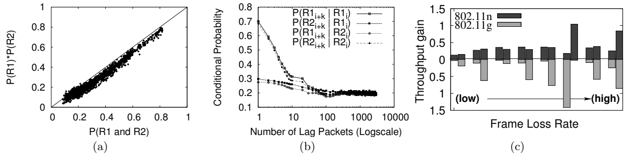
Figure 8: (a) P_l(R_1 \cap R_2) \approx P_l(R_1) * P_l(R_2) indicates that the losses are largely independent across receivers R_1 and R_2 . (b) Auto-conditional and cross-conditional packet error probabilities for broadcast experiments performed using two 802.11n receivers. (c) Throughput gains when using MAC-diversity with two receivers for 802.11n and 802.11g.
