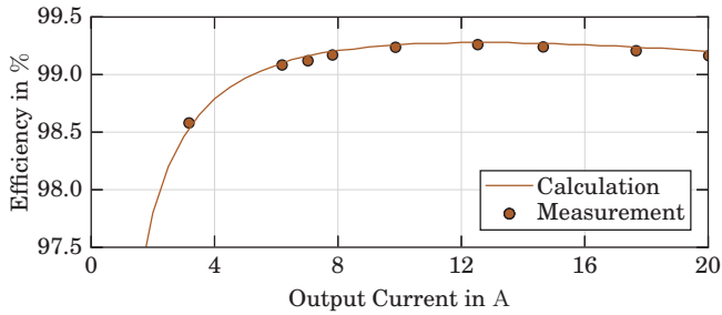
Fig. 11. Calculated and measured efficiency of the rectifier as function of I_1 , indicating that the converter achieves an efficiency above 99% for > 30% load with peak efficiency of 99.26%. Measurements were taken on the prototype shown in Fig. 9 using a Yokogawa WT3000 power analyzer.
