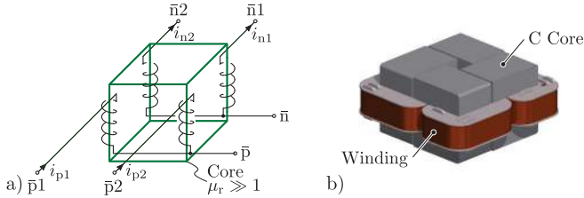
Fig. 7. (a) Structure of the implemented symmetrical, cube-type ICMCI core which is constructed from four C cores with one winding each as shown in (b).
