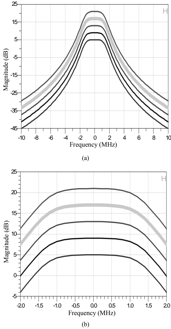
Figure 5. Frequency response of the third order low-pass filter. (a) Total response; (b) Zoom in on the pass band of the frequency response
