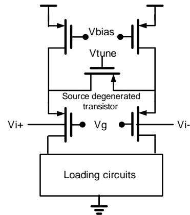
Figure 1. The input stage of the proposed bulk driven transconductance.
