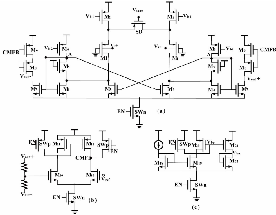
Figure 2. The complete OTA (a) The transconductance main stage; (b) The CMFB circuit; (c) The bias circuit.
