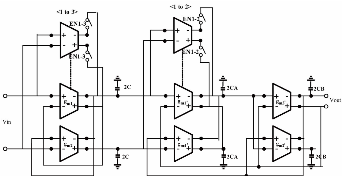
Figure 3. The implementation of the third order low-pass filter.
