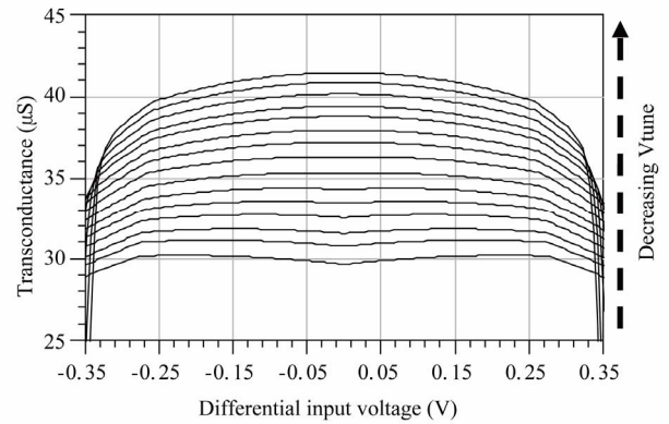
Figure 4. Transconductance tuning versus differential input voltage.
