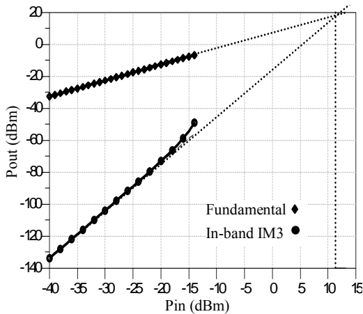
Figure 6. In-band IIP_3 calculation for a 5 dB gain of the filter.
