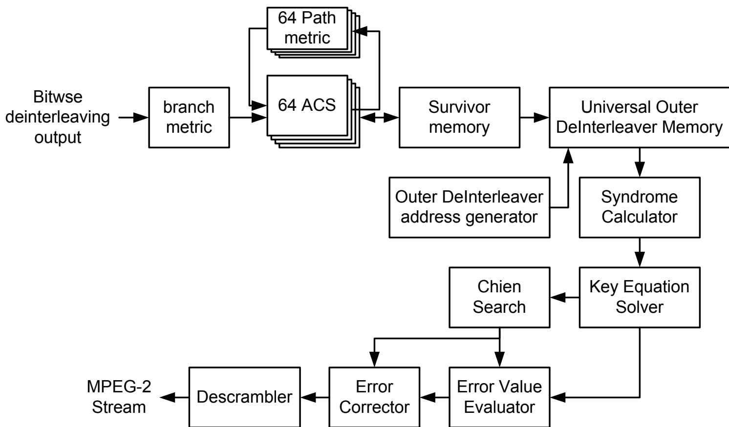
Figure 14.6.4: FEC architecture for DVB-T/H system.
