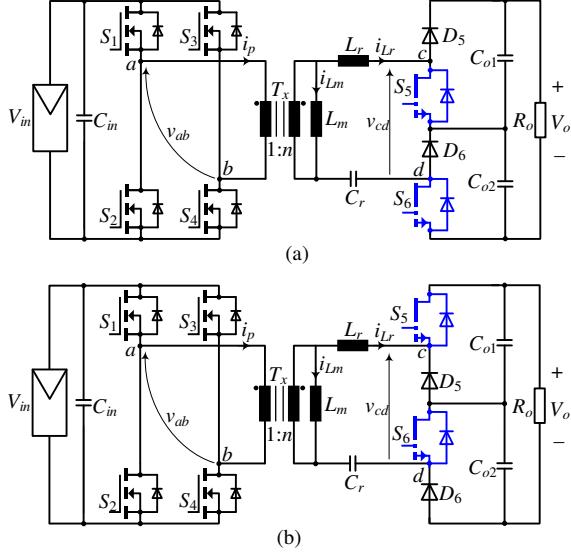
Fig. 3. Schematics of the extended series resonant converter topologies with dual-mode rectifiers for high-voltage output applications: (a) extended topology A and (b) extended topology B.
