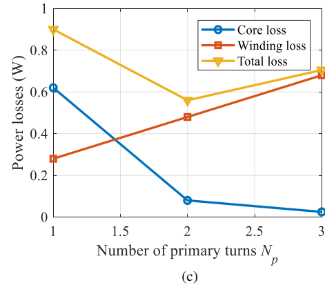
Fig. 18. Calculated power losses of planar transformers with different winding arrangements and different numbers of primary turns N_p : (a) non-interleaving winding arrangements: P-S for N_p = 1 , P-P-S-S for N_p = 2 , P-P-P-S-S-S for N_p = 3 , (b) interleaving winding arrangement: P-S for N_p = 1 , P-S-P-S for N_p = 2 , P-S-P-S-P-S for N_p = 3 , (c) 0.5P-S-0.5P for N_p = 1 , 0.5P-S-P-S-0.5P for N_p = 2 , 0.5P-S-P-S-P-S-0.5P for N_p = 3 .
