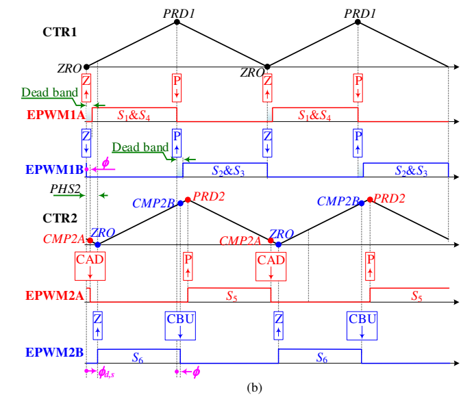
Fig. 23. Modulation waveforms based on TMS320F28075 DSP (a) \phi > \phi_{d,s} , (b) \phi \leq \phi_{d,s} . PRD1 and PRD2 represent the period registers of the two ePWM modules (ePWM1 and ePWM2), PHS2 is the phase register of ePWM2, CMP2A and CMP2B are the counter-compare A and B registers of ePWM2. CAU indicates the event when the counter CTR2 equals the active CMP2A register and CTR2 is incrementing. CAD indicates the event when the counter CTR2 equals the active CMP2A register and CTR2 is decrementing. CBU indicates the event when the counter CTR2 equals the active CMP2B register and CTR2 is incrementing. CBD indicates the event when the counter CTR2 equals the active CMP2B register and CTR2 is decrementing. Z and P represents the events when the counter equals zero and the period, respectively.
