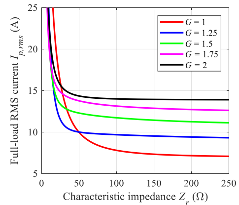
Fig. 9. Full-load RMS currents with respect to the characteristic impedance Z_r at different voltage gains. (a) Secondary-side RMS current I_{Lr,rms} ; (b) Primary-side RMS current I_{p,rms} .
