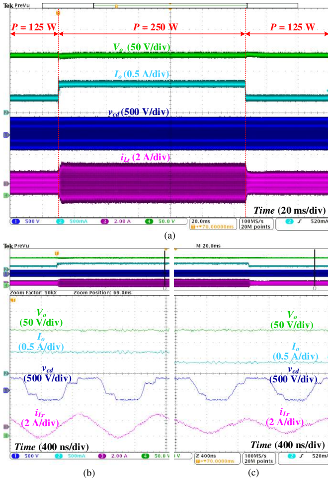
Fig. 26. Transient performance of the proposed converter with the output voltage closed-loop control (the input voltage V_{in} = 30 V and the output voltage reference V_{o,ref} = 340 V): (a) transition between P = 250 W and P = 125 W, (b) zoomed-in waveforms at P = 250 W, (c) zoomed-in waveforms at P = 125 W.
