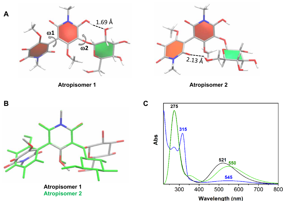
Fig. 4. Analysis of the thermodynamically favored atropisomers of chrozophoridin, in solution. Molecules are depicted as sticks and colored by atom type. (A) A ring, B ring, and glucose ring are colored in red, orange, and green, respectively. Both \omega_1 and \omega_2 dihedrals and hydrogen bonds are also indicated. (B) Superposition of the A ring of the two molecules. Colored by element (atropisomer 1) and green (atropisomer 2). (C) UV-VIS spectra (water, pH 7, blue) for chrozophoridin compared with the predicted spectra [Boese-Martin for kinetics (BMK) functional] for atropisomers 1 (black) and 2 (green).
