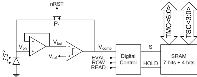
Fig. 2: TS Pixel Block Diagram
