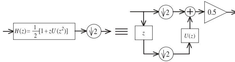
Fig. 4. Lifting update implementation of a half-band filter.
