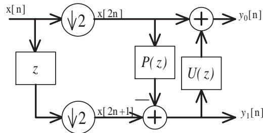
Fig. 1. Lifting analysis stage.
