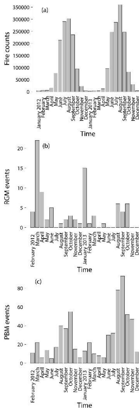
Figure 5. (a) Fire counts west of Amsterdam Island (latitude: 3\text{--}53^\circ \text{ S} , longitude: 10\text{--}73^\circ \text{ E} ) in 2012 and 2013. Data courtesy of FIRMS MODIS Fire Archive Download. (b) RGM events, i.e., number of measurements above quantification limit, at Amsterdam Island from February 2012 to December 2013. (c) PBM events, i.e., number of measurements above quantification limit, at Amsterdam Island from February 2012 to December 2013.
