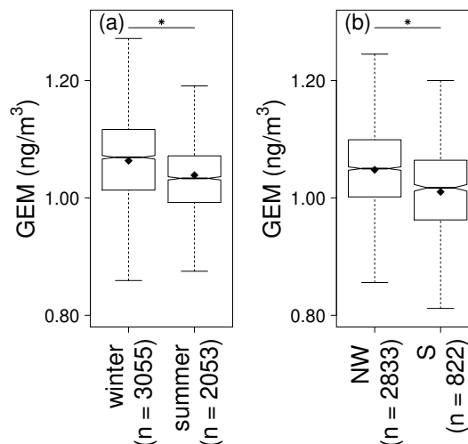
Figure 4. Hourly average GEM concentrations ( \text{ng m}^{-3} ) measured at Amsterdam Island: (a) in winter (July–September) or summer (December–February) and (b) under NW or S winds. \blacklozenge : mean, *: statistically significant difference, n = number of hourly average data, bottom and top of the box: first and third quartiles, band inside the box: median, ends of the whiskers: lowest (highest) datum still within the 1.5 interquartile range of the lower (upper) quartile. Outliers are not represented
