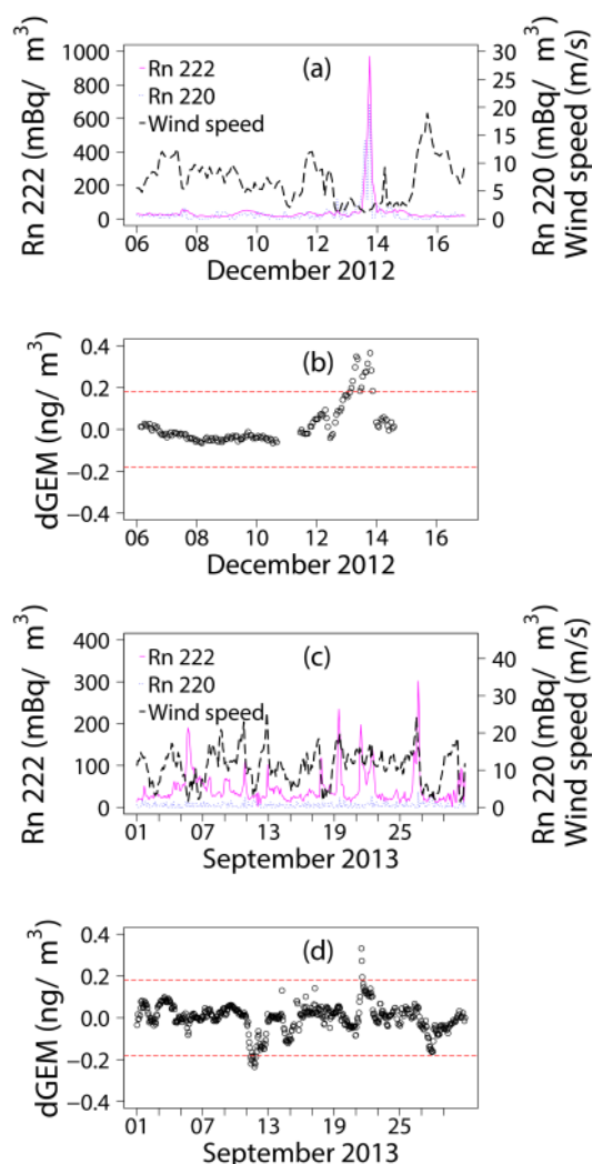
Figure 6. Examples of ^{222}\text{Rn} ( \text{mBq m}^{-3} ) peaks observed at Amsterdam Island along with ^{220}\text{Rn} ( \text{mBq m}^{-3} ) activity and wind speed ( \text{m s}^{-1} ) (a) in December 2012 and (c) in September 2013. Background variability (dGEM; \text{ng m}^{-3} ) of GEM concentrations observed at Amsterdam Island in (b) December 2012 and (d) September 2013. Dotted lines represent 3 times the mean monthly standard deviation of dGEM measurements.
