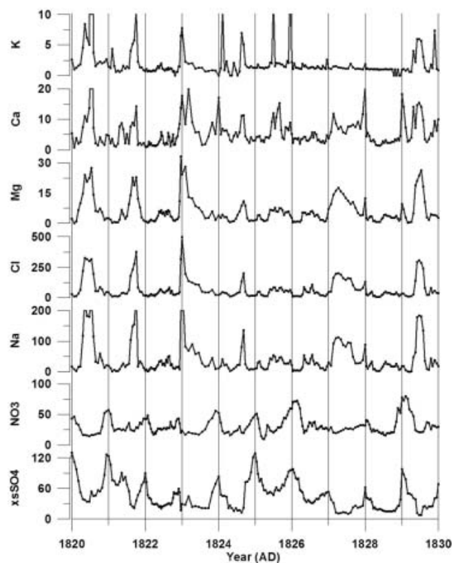
Fig. 2. Raw ion data from core 01-5 plotted vs time. Ion concentrations are in parts per billion. These data are from 94–99 m depth (AD 1820–30) in the core. Vertical lines represent 1 year increments.
