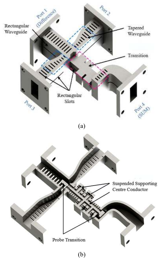
Fig. 1. Structural illustrations of the proposed monolithically integrated E -plane waveguide magic-T using air-filled rectangular-coax-to-waveguide transitions. (a) The complete fabrication model. (b) The E -plane profile showing the internal geometry.
