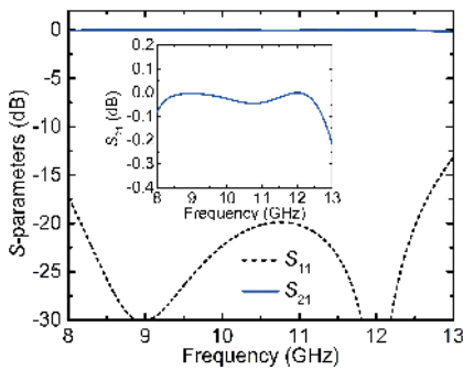
Fig. 3. EM-simulated S -parameters of the designed X-band air-filled rectangular coaxial TL. The electrical conductivity of 5.96 \times 10^7 S/m was used for copper boundaries.
