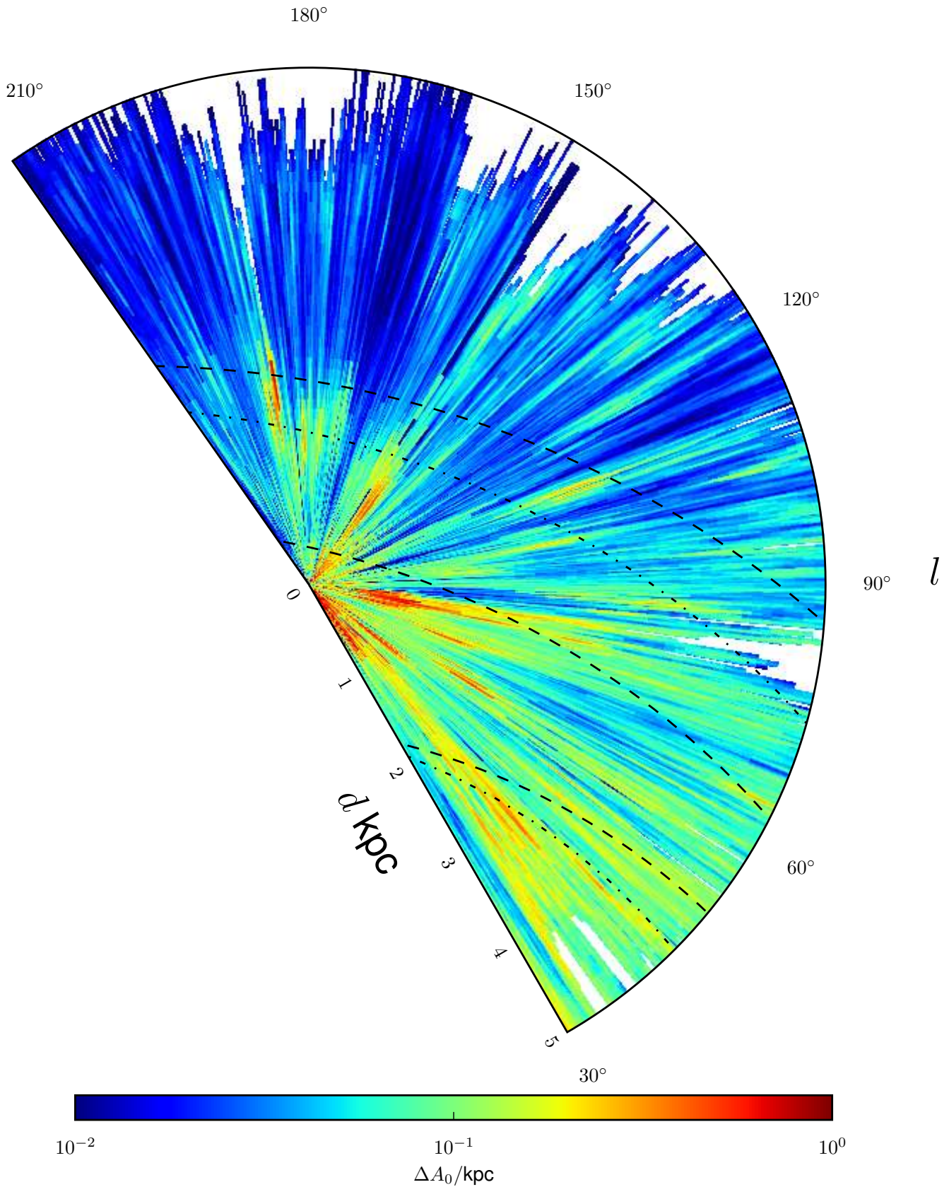
Figure 5. A map of extinction at b = 0 , after convolution with a uniform kernel to reduce the resolution to 0.25^\circ in l and 500 pc in distance, so as to roughly match the resolution of Figure 9 of Marshall et al. (2006). The sun lies at the plot's origin with the Galactic centre off the bottom of the plot. The dashed lines denote the position of the Sagittarius, local and Perseus spiral arms given by Reid et al. (2014), whilst the dot-dashed lines correspond to the Sagittarius and Perseus arms of Vallée (2013). Note the nonphysical 'fingers of God' – discontinuities in the azimuthal direction.
