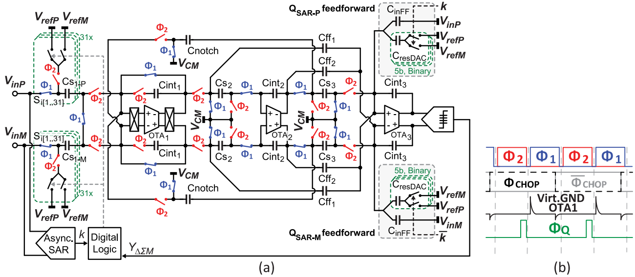
Fig. 9. Simplified circuit diagram of (a) proposed DT zoom ADC, with the corresponding timing diagram and simplified visualization of the virtual ground of OTA1 due to (b) switching activities.
