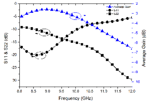
Fig. 6. Measured input/output return losses and average gain of the vector-sum phase shifter.
