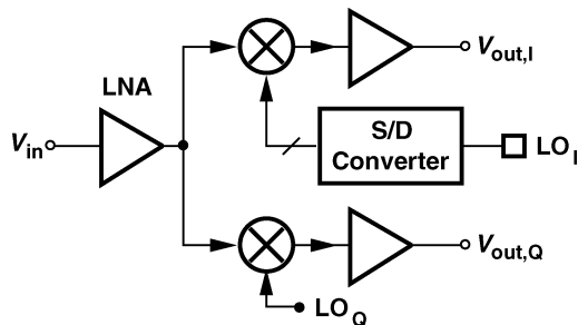
Fig. 1. Receiver architecture.
