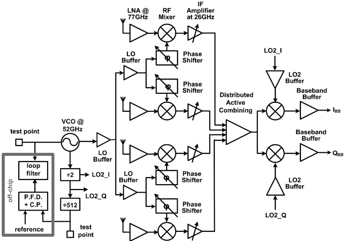
Fig. 12. System architecture.
