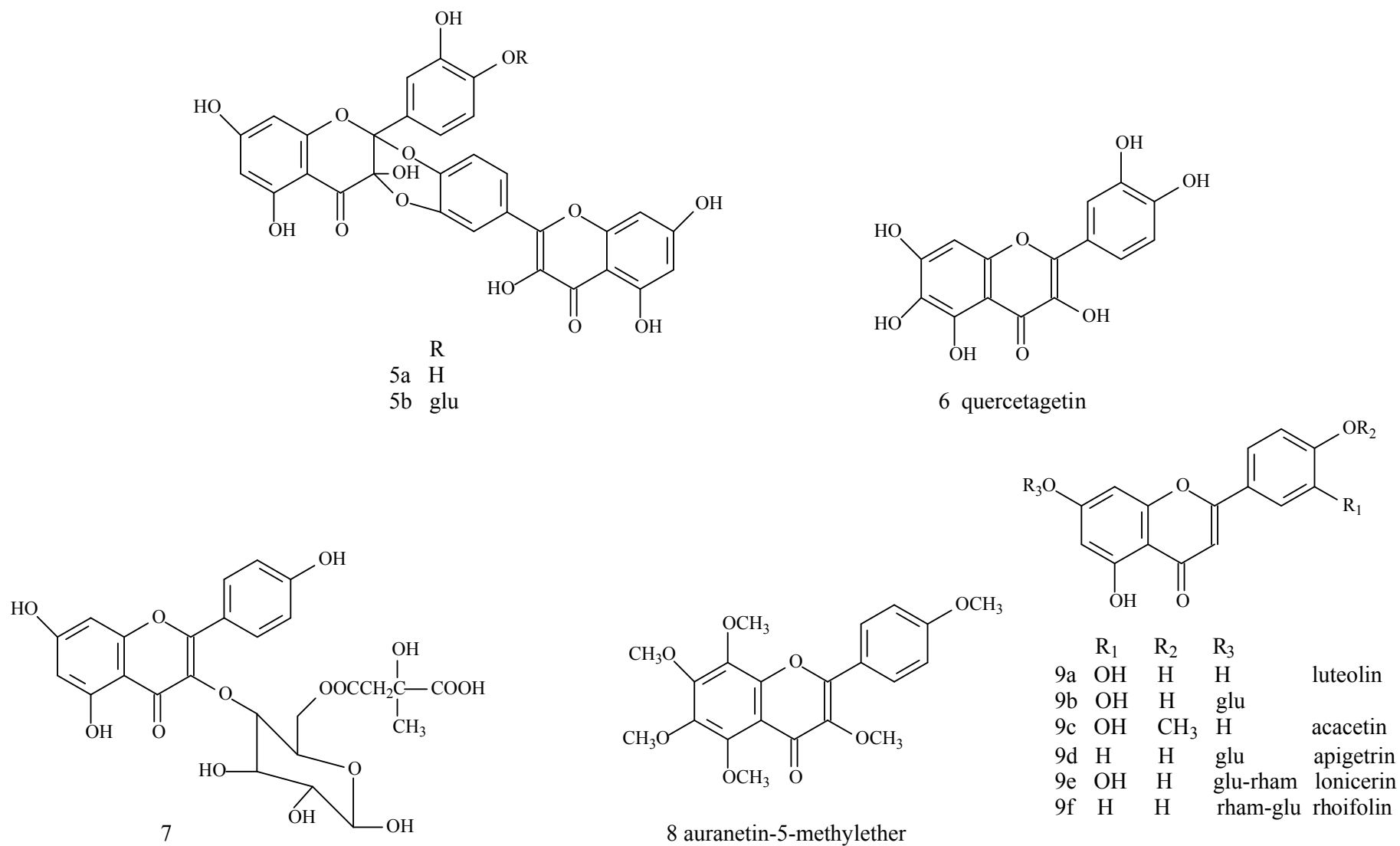
Figure 2. Flavonoids presenting \alpha -amylase inhibition activity (..... Continued)
