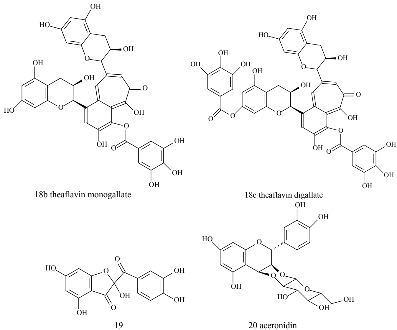
Figure 2. Flavonoids presenting \alpha -amylase inhibition activity (Continued)
