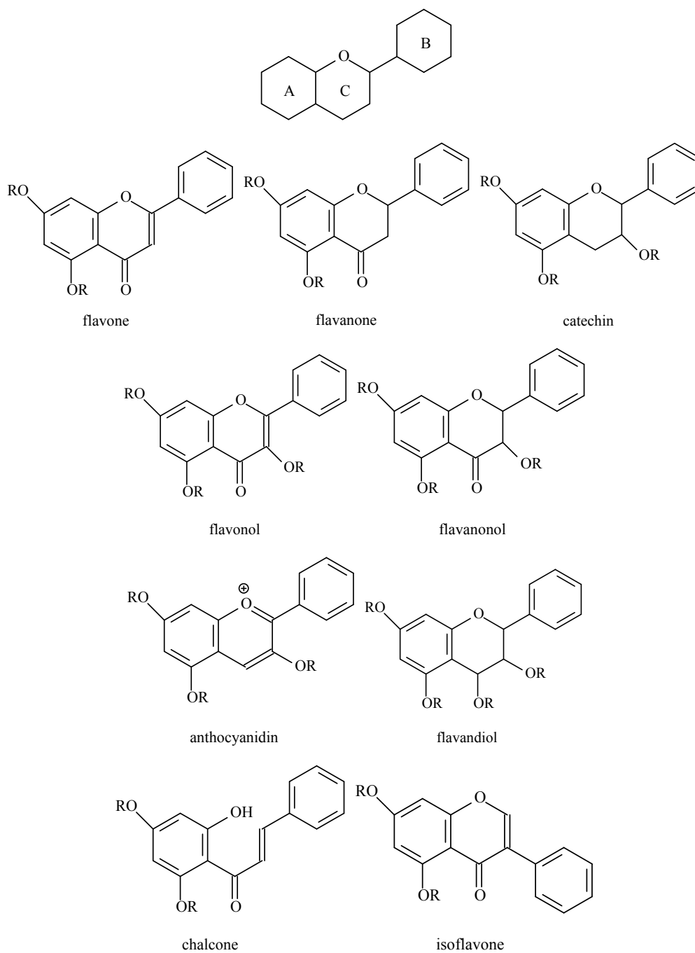
Figure 1. Flavonoids basic skeletons
