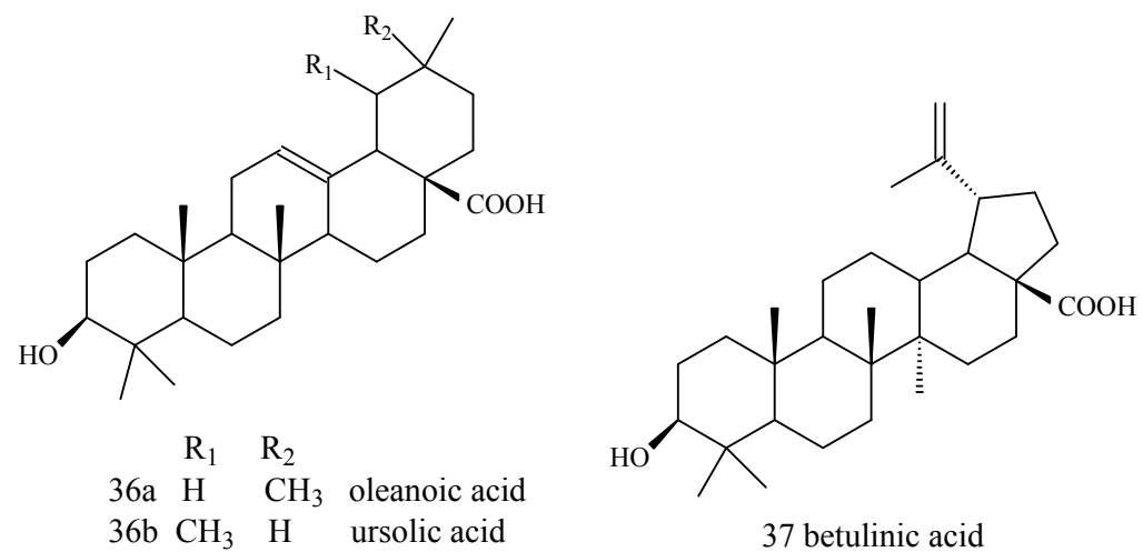
Figure 5. Terpenes presenting \alpha -amylase inhibition activity (Continued....)
