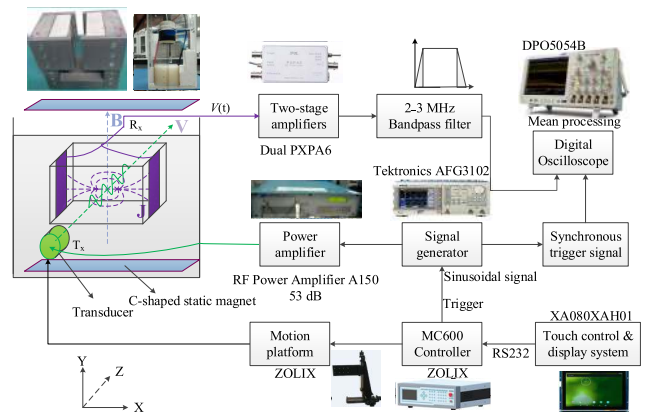
FIGURE 2. Connection schematic of proposed MAET system.
