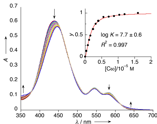
Figure 2. Concentration dependence of the UV-vis absorption spectra: [4Ni] = 2.0 \mu\text{M} , [ \text{C}_{60} ] = 0–16 \mu\text{M} , toluene, 25°C. Inset: a titration curve of 4Ni under various concentration of [ \text{C}_{60} ].
