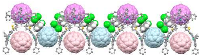
Figure 4. A columnar array of the fullerene molecules along the a -axis shown as a space-filling model. For clarity, 4Ni units are shown as a ball-and-stick model. The blue C 60 molecules directly interconnect face-to-face with two (C 60 ) 2 @ 4Ni , and purple C 60 molecules through the two dichlorobenzene molecules. tert -Bu groups are omitted for clarity.
