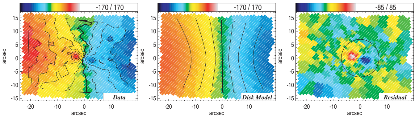
Figure 3. A thin isothermal disc model for the stellar velocity field of NGC 5448. The circle marks the 7-arcsec region within which we find a disc-like structure. The disc model, fitted to the field outside this region, implies for the outer disc a scalelength of 18 arcsec, V_{\text{sys}} = 2002 \text{ km s}^{-1} , and PA = 91^\circ . The orientation of the maps is the same as in Fig. 1.
