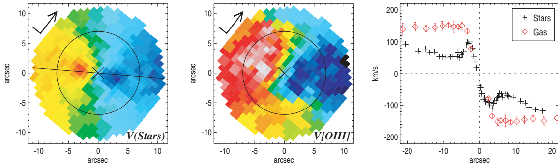
Figure 6. Zooming into the central few arcsec of the stellar and gaseous velocity maps of NGC 5448, using the same velocity range as in Fig. 1. Indicated are the north–east direction (arrow), the photometric PA (straight line) and the photometric centre (cross). The overlapped circle indicates the 7-arcsec radius for comparison with Fig. 3. In the right panel, we present the stellar rotation curve (extracted along the photometric PA) together with the gas rotation curve derived from tilted-ring decomposition.
