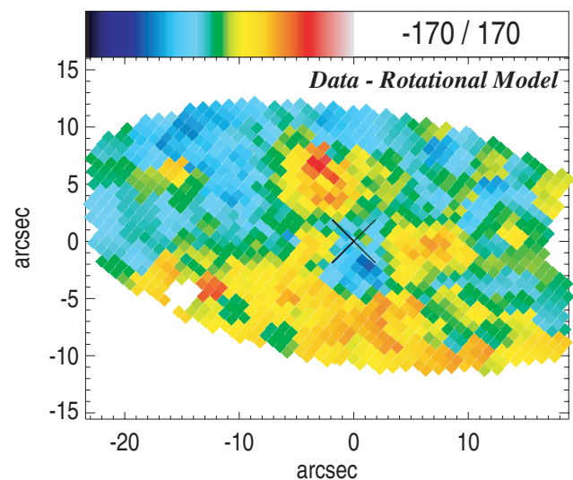
Figure 7. Residual field after subtracting the best-fitting rotational model from the observed gas velocity field. This map reveals the strong non-circular motions in NGC 5448, however, no ring-like feature is found.
