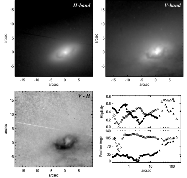
Figure 5. The top panels show HST /NICMOS H -band (F160W) and WFPC2 V -band (F606W) images of NGC 5448. The bottom-left panel is the V – H map obtained by convolving the H -band image with the V -band image point spread function (PSF) and vice versa, and subtracting one from the other. All maps have pixel size of 0.0455 arcsec, and the same orientation as the DSS image with the centre marked by a cross. The bottom-right profiles are the observed (open symbols) and deprojected (filled symbols) ellipticity and PA profiles from Laine et al. (2002). Circles represent values derived from the NICMOS image, and triangles show the values derived using the DSS image. Here, we only focus on the region beyond 1 arcsec.
