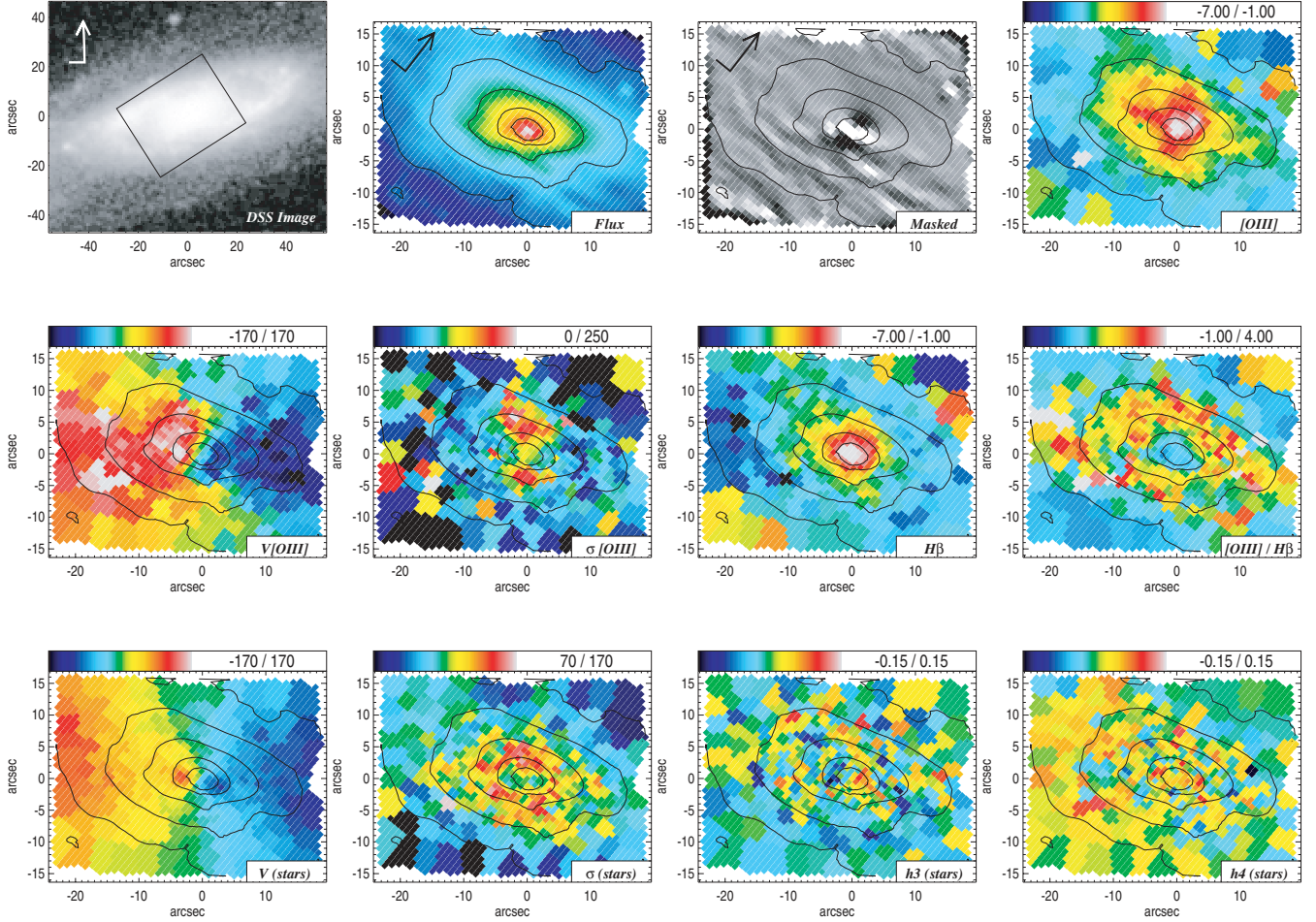
Figure 1. Top left: Digitized Sky Survey image with SAURON footprint and north–east orientation arrow. All other panels show the SAURON data. The stellar flux map and unsharp-masked SAURON image are given in \text{mag arcsec}^{-2} with arbitrary zero point, and north–east direction as indicated. The titles are indicated at the bottom-right corner of each panel with plotting ranges according to the top colour bar. All SAURON maps have the same orientation with overlapped stellar contours in magnitude steps of 0.25, and all velocities and velocity dispersions are given in \text{km s}^{-1} .
