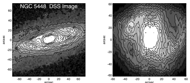
Figure 8. Observed (left) and deprojected (right) DSS image of NGC 5448. The inclination of 64^\circ and PA of 115^\circ from the RC3 catalogue have been used to deproject the image according to the two-dimensional deprojection of a circular thin disc.
