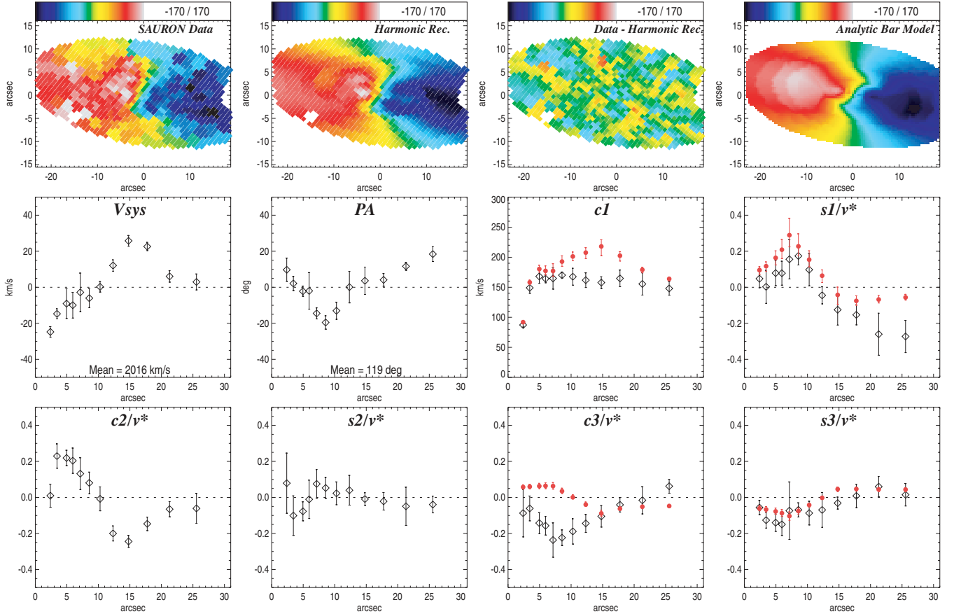
Figure 2. Top row, from left to right: observed SAURON gas velocity field of NGC 5448; reconstruction based on the harmonic decomposition of the SAURON gas velocity field; residual field (data – harmonic reconstruction); and the analytic bar model, which reproduces best the main kinematic features of the observed gas velocity field. Middle and bottom row: the harmonic parameters as a function of outer radius of each ring, and v^* = c_1 \sin i . The overplotted red filled circles are the analytically calculated first and third harmonic terms for the bar model (the second terms are zero by construction), with the error bars corresponding to the 3\sigma (99.7 per cent) confidence level (see Section 4 for details). The orientation of the maps is the same as in Fig. 1, and the mean PA value is given in the north–east direction.
