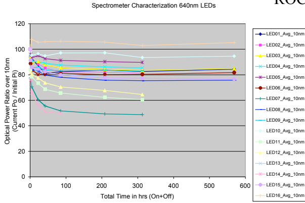
Fig 1 ALT for Batch2, 483mA
