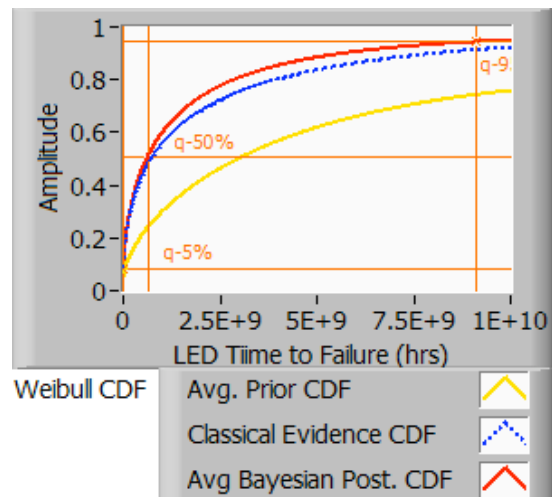
Fig 6. 2 nd Average Predictive Posterior of LED TTF
