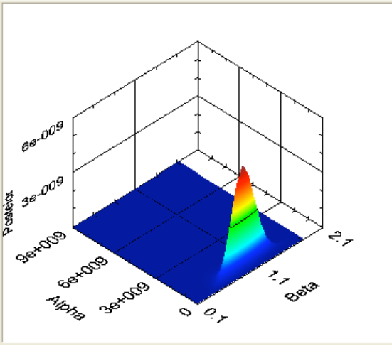
Fig 3. 1 st Posterior Joint \alpha - \beta distribution for AlGaInP-MQW-Pulse-Transformed
