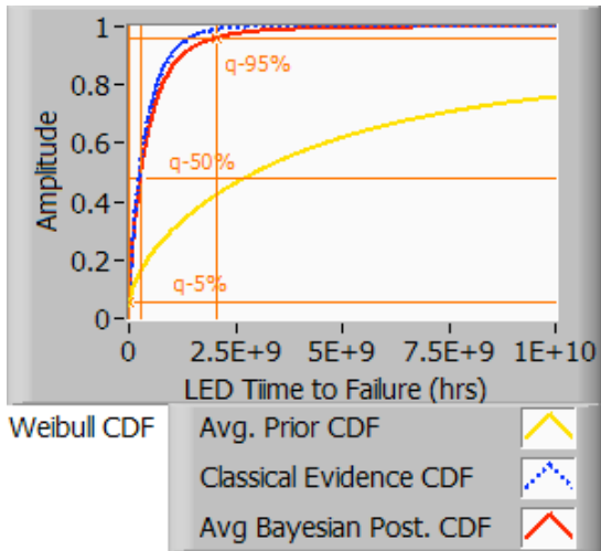
Fig 4. 1 st Average Predictive Posterior of LED TTF
