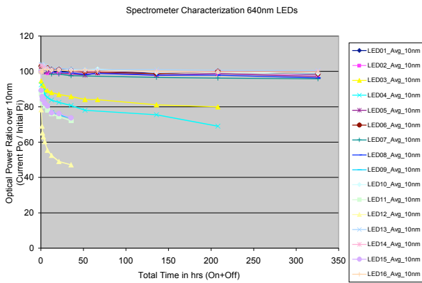
Fig 2 ALT for Batch3, 725mA
