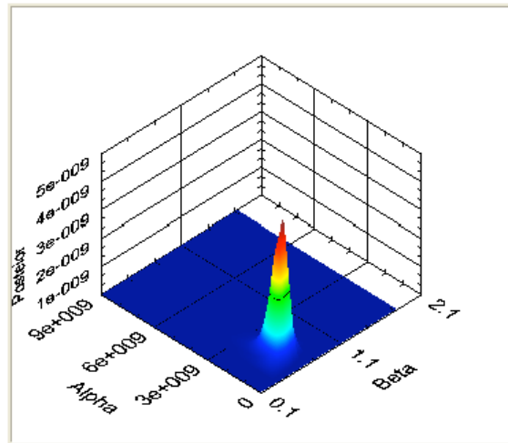
Joint Alpha Beta Posterior Distribution
