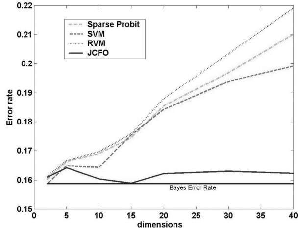
Fig. 1. Effect of increasing numbers of irrelevant features added to a series of synthetic data sets. In accordance with the curse of dimensionality, the error rate of most kernel classifiers increases as more irrelevant features are introduced, but our JCFO algorithm is largely immune.
