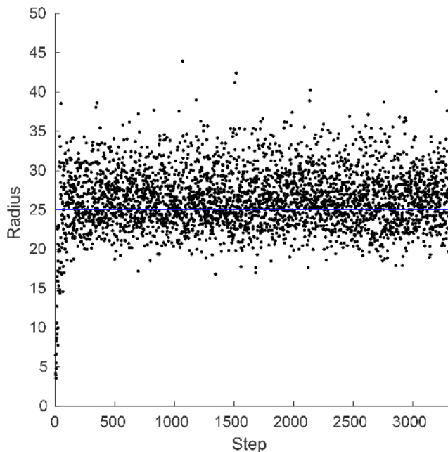
Figure 10. QGSO sample radii. For the configuration in Fig. 8 with \alpha = 1.08 , \bar{\nu} = 25 , and \text{Var}(\nu) = 4 . Each dot represents a radius, with the line representing the mean.
