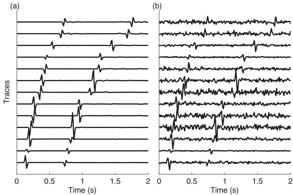
Figure 10. Example vertical component synthetic data for a double-couple source with added Gaussian noise. (a) shows the synthetic data, and (b) the same data with the added noise with an SNR of 3. The frequency content of the signal is band-pass filtered between 1 and 40 Hz.
