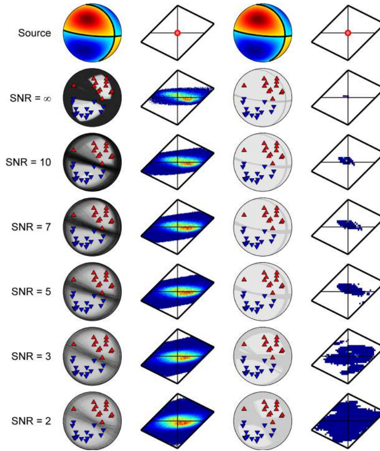
Figure 12. Lower hemisphere equal area projections and Hudson plots of the source PDF for a synthetic double-couple source for a range of data uncertainties, corresponding to \text{SNR} = \infty , \text{SNR} = 10 , \text{SNR} = 7 , \text{SNR} = 5 , \text{SNR} = 3 and \text{SNR} = 2 . The first and third columns show the source PDF for the solution constrained to be double-couple only. The second and fourth columns show the source PDF for the full moment tensor solution. The first two columns show the solutions for inversions using only polarity data, and the second two columns show the solutions using polarity and amplitude ratio data. Manually picked station first motions are given by upward red or downward blue triangles. For the focal sphere plots, possible fault planes are given by dark lines. The most likely fault planes are given by the darkest lines. For the Hudson plots, high probability is red and low probability is in blue. The positions of the different source types on the Hudson plot are shown in Fig. 9. The posterior model probabilities for the double-couple source model determined from the Bayesian evidence are, from top to bottom, 0.77, 0.78, 0.80, 0.84, 0.91 and 0.94, for the polarity only inversion, and 1.0, 0.01, 0, 0, 0.02 and 0.01, for the polarity and amplitude ratio inversions.
