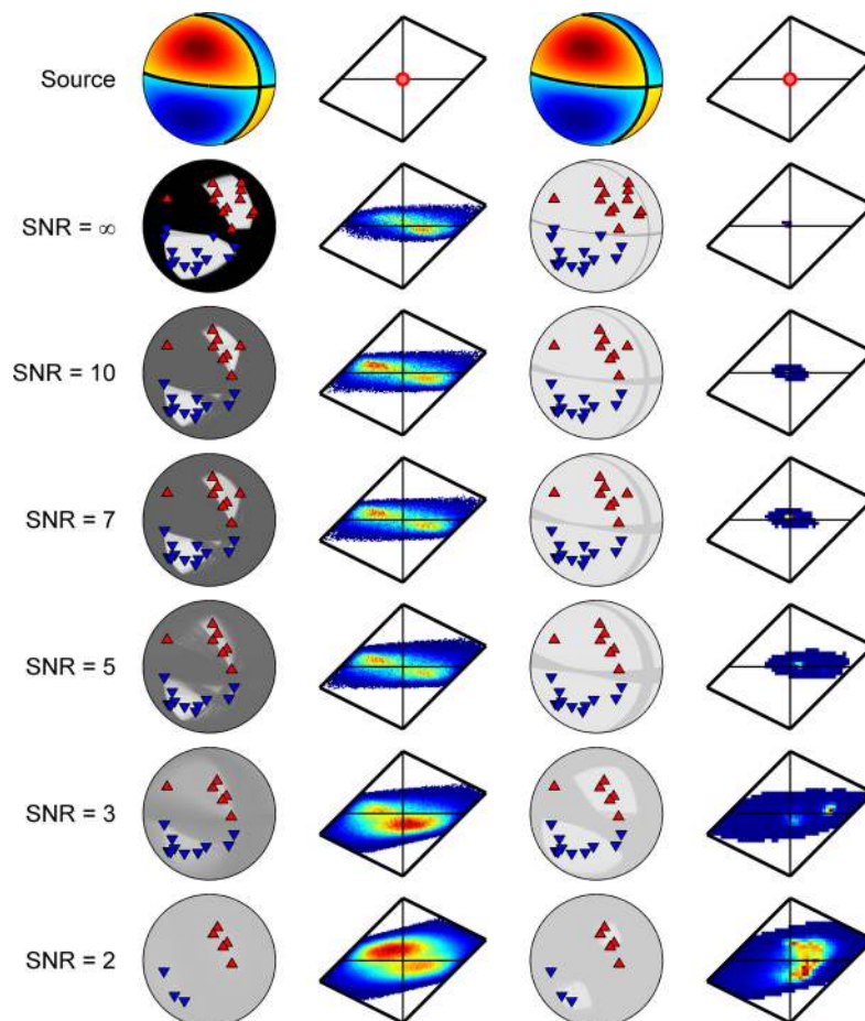
Figure 13. Lower hemisphere equal area projections and Hudson plots of the source PDF for a synthetic double-couple source with a range of noise levels, \text{SNR} = \infty , \text{SNR} = 10 , \text{SNR} = 7 , \text{SNR} = 5 , \text{SNR} = 3 and \text{SNR} = 2 . The first and third columns show the source PDF for the solution constrained to be double-couple only. The second and fourth columns show the source PDF for the full moment tensor solution. The first two columns show the solutions for inversions using only polarity data, and the second two columns show the solutions using polarity and amplitude ratio data. Manually picked station first motions are given by upward red or downward blue triangles. For the focal sphere plots, possible fault planes are given by dark lines. The most likely fault planes are given by the darkest lines. For the Hudson plots, high probability is red and low probability is in blue. The positions of the different source types on the Hudson plot are shown in Fig. 9. The posterior model probabilities for the double-couple source model determined from the Bayesian evidence are, from top to bottom, 0.77, 0.71, 0.71, 0.77, 0.64 and 0.62, for the polarity only inversion, and 0, 0.99, 0.70, 0.84, 0.82 and 0.58, for the polarity and amplitude ratio inversions.
