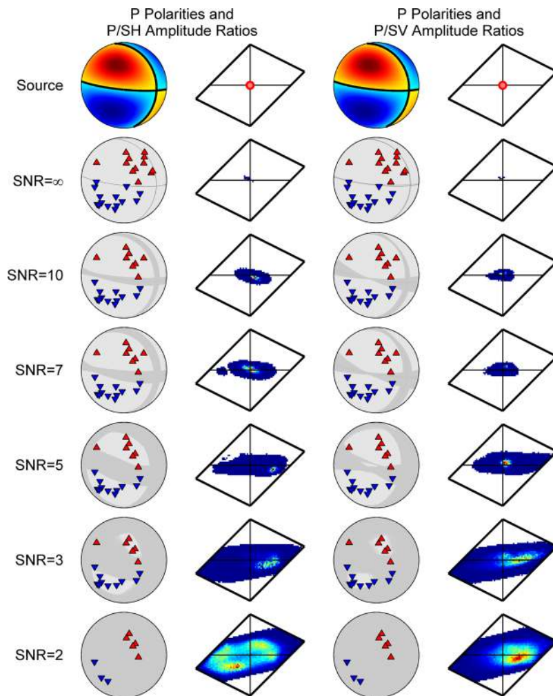
Figure 14. Lower hemisphere equal area projections and Hudson plots of the source PDF for a synthetic double-couple source using P polarity and either P/SH - or P/SV -amplitude ratios. The first and third columns show the source PDF for the solution constrained to be double-couple only. The second and fourth columns show the source PDF for the full moment tensor solution. Manually picked station first motions are given by red (up) or blue (down) points, with darker points corresponding to more likely locations. For the focal sphere plots, possible fault planes are given by dark lines. The most likely fault planes are given by the darkest lines. For the Hudson plots, high probability is red and low probability is in blue. The positions of the different source types on the Hudson plot are shown in Fig. 9.
