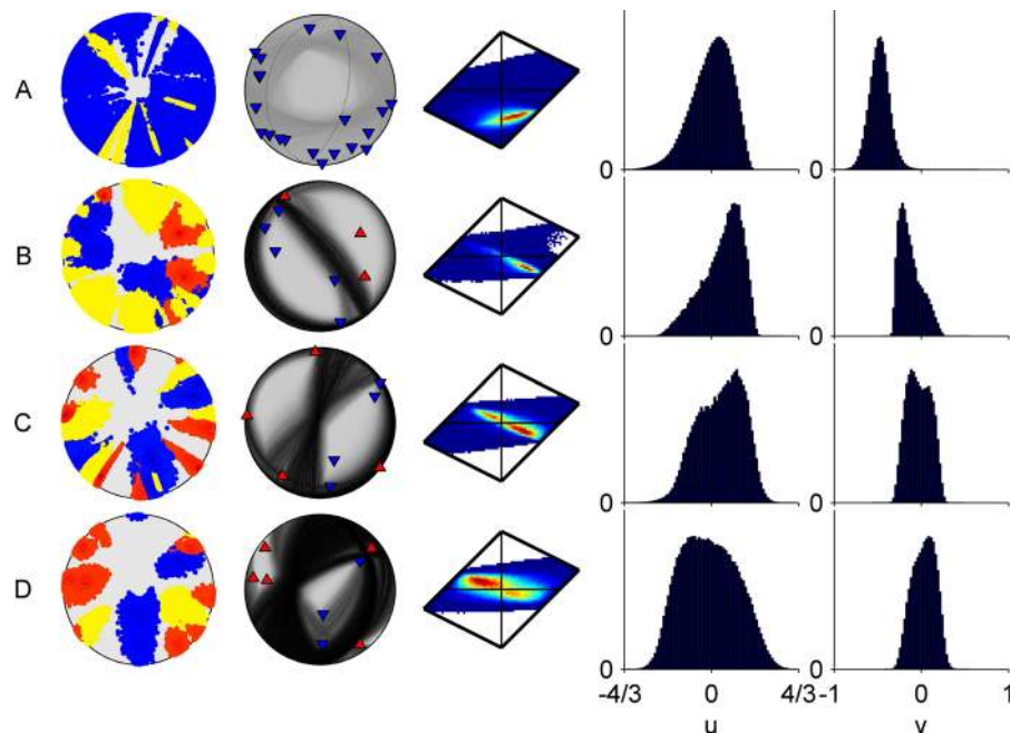
Figure 19. Lower hemisphere equal area projections, Hudson plots and marginalized distributions of the Hudson u and v parameters of four events from the Krafla geothermal region of Iceland. The first column shows the station ray position distribution from the NonLinLoc location PDF. The second column shows the maximum likelihood location station positions and the source PDF for the solution constrained to be double-couple only. The third column shows the source PDF for the full moment tensor solution. The fourth and fifth columns show the marginalized distributions of the Hudson u and v parameters, respectively. Manually picked station first motions are given by red (up) or blue (down) markers, with darker points corresponding to more likely locations in the ray position distribution. For the focal sphere plots, possible fault planes are given by dark lines. The most likely fault planes are given by the darkest lines. For the Hudson plots, high probability is red and low probability is in blue. The positions of the different source types on the Hudson plot are shown in Fig. 9. The posterior model probabilities for the double-couple source model determined from the Bayesian evidence and the Bayesian information criterion values are both given in Table 3.
