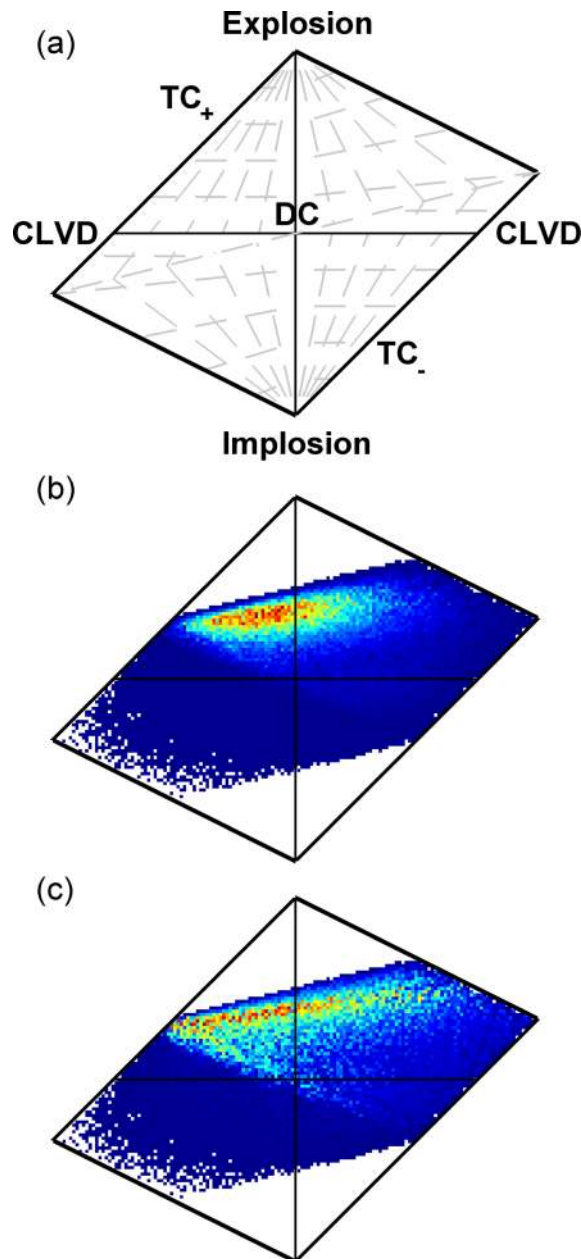
Figure 9. Comparison of marginalized and silhouette plots of the source PDF types for an example real event. (a) shows the position of different source types on the Hudson plot, with the double-couple point located where the axes cross. Several source types are shown on the plot: the compensated linear vector dipole (CLVD) end members (Knopoff & Randall 1970), the implosive and explosive sources, the positive and negative tensile crack sources ( TC_+ and TC_- ) for a Poisson's ratio of 0.25, and the double-couple source (DC). (b) shows the marginalized source PDF, and (c) the silhouette plot of the source PDF for the equal area Hudson plot. Red shows high probability, and blue low (non-zero) probability.
