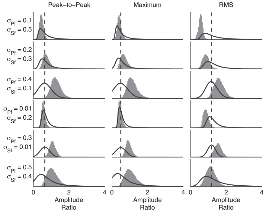
Figure 4. Histogram of amplitude ratio distributions (in grey) with differing fractional noise levels for the P , \sigma_{Pf} , and S , \sigma_{Sf} , arrivals using different measurement approaches. The vertical dashed lines correspond to the correct values and the solid lines are the assumed distributions of the observed ratios given the correct amplitudes and uncertainties, corresponding to the ratio PDF as defined in Section 4.3.2. The fractional noise corresponds to the inverse of the true SNR value. The vertical scales are independent between the plots because the amplitude ratio distributions are normalized so that the area integral is 1.
