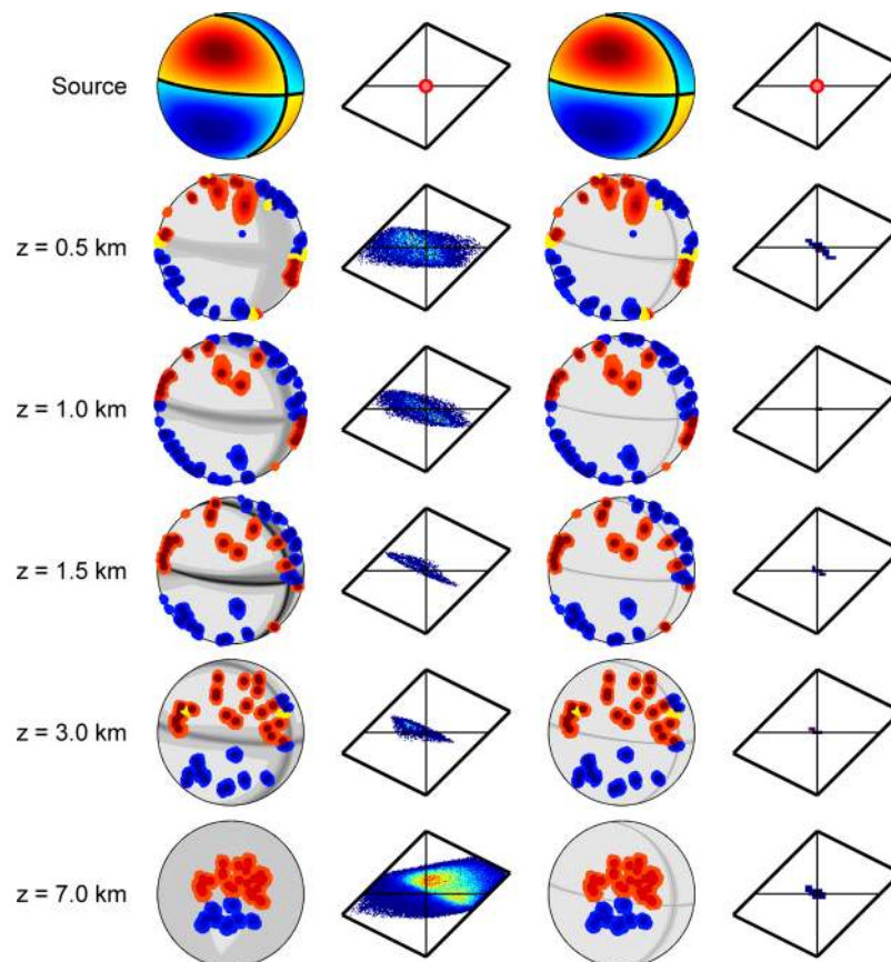
Figure 15. Lower hemisphere equal area projections and Hudson plots of the source PDF, marginalized over the location uncertainty, for a synthetic double-couple source at a range of source depths in the centre of an array, z = 0.5 km, z = 1 km, z = 1.5 km, z = 3 km and z = 7 km. The first and third columns show the scatter of station ray positions on the focal sphere for the NonLinLoc location PDF and the source PDF for the solution constrained to be double-couple only. The second and fourth columns show the source PDF for the full moment tensor solution. The first two columns show the solutions for inversions using only polarity data, and the second two columns show the solutions using polarity and amplitude ratio data. Manually picked station first motions are given by red (up) or blue (down) points, with darker points corresponding to more likely locations. For the focal sphere plots, possible fault planes are given by dark lines. The most likely fault planes are given by the darkest lines. For the Hudson plots, high probability is red and low probability is in blue. The positions of the different source types on the Hudson plot are shown in Fig. 9. The posterior model probabilities for the double couple source model determined from the Bayesian evidence are, from top to bottom, 0.80, 0.91, 0.74, 0.95 and 0.38, for the polarity only inversion, and 0.99, 0, 1, 1 and 1, for the polarity and amplitude ratio inversions.
