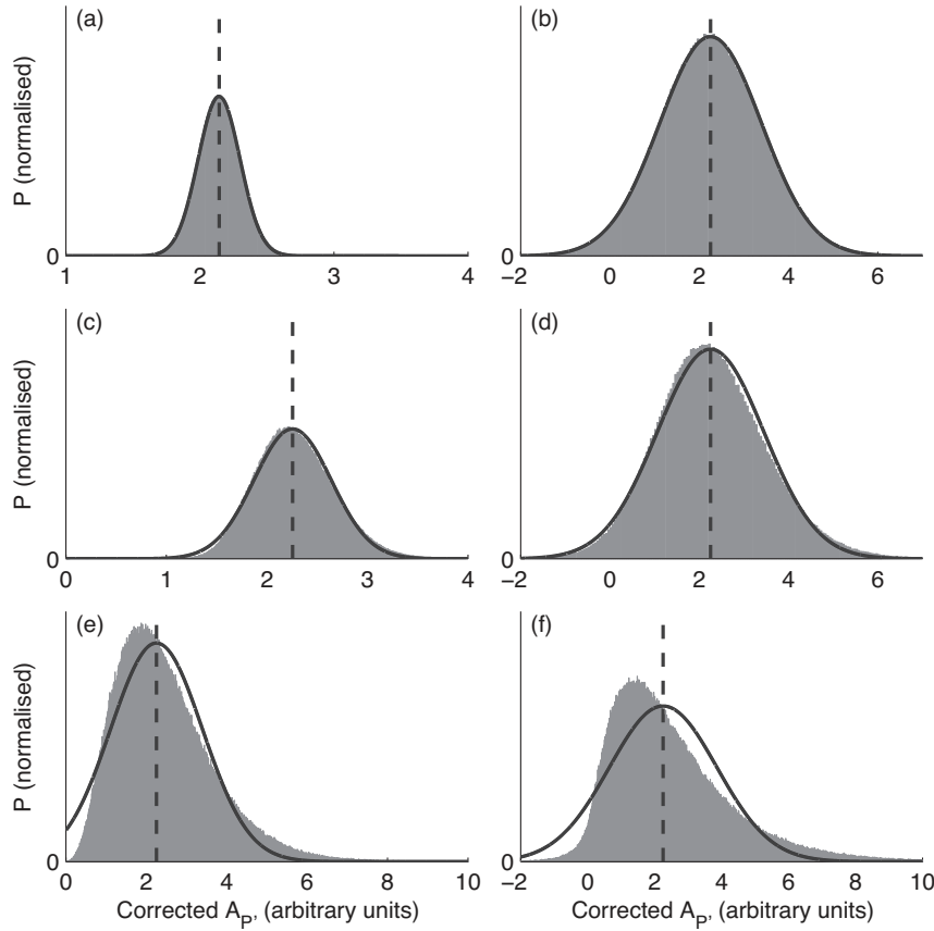
Figure 6. Histograms of the propagation corrected model P amplitude A_p distributions (in grey). The solid lines correspond to \mathcal{N}(A_p, \mu_{A_p}, \sigma_{A_p}) calculated according to eqs (34) and (35). The dashed vertical lines correspond to \mu_{A_p} , and the histograms show the actual distribution calculated from 1 000 000 samples from Gaussian distributions for A_p and V_p/V_S with \mu_{V_p/V_S} = 1.75 . The left column shows the distributions for a P amplitude SNR = 40, the right column SNR = 2. (a) and (b) \sigma_{V_p/V_S} = 0.04 , (c) and (d) \sigma_{V_p/V_S} = 0.1 , and (e) and (f) \sigma_{V_p/V_S} = 0.3 . The vertical scales are independent between the plots as the amplitude distributions are normalized so that the area integral is 1.
