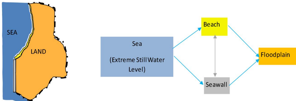
Figure 2: Left: Land-use map of a generic coastal floodplain; Right: Quasi-2D SPR system diagram for floodplain (blue arrows show hydraulic links, grey arrow shows morphological influence)
