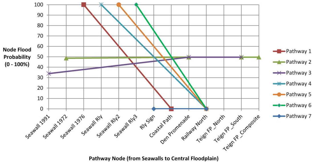
Figure 12: Flood probabilities of network nodes along all open coast pathways numbered in Figure 11
