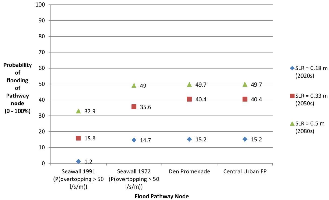
Figure 13: Node flood probabilities versus sea-level rise, for pathways 2 and 3, for ‘unknown’ Sediment Input
