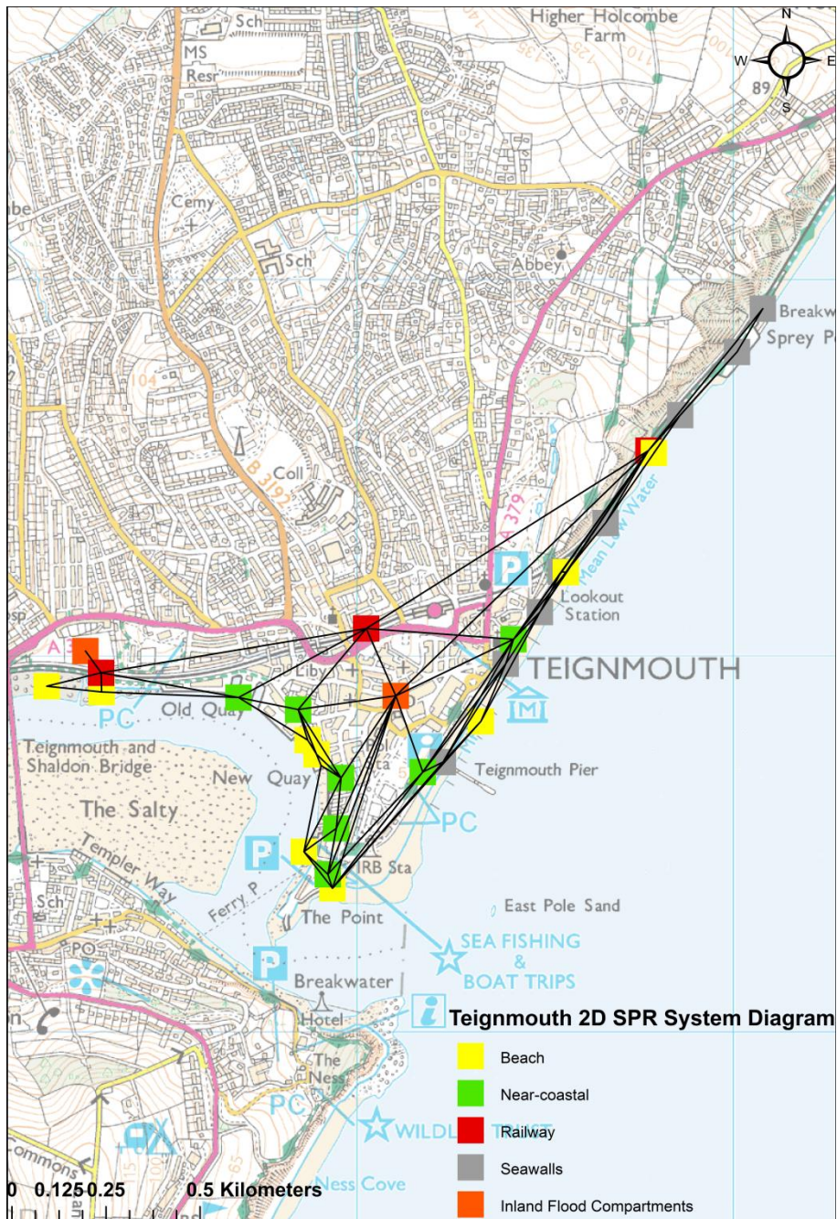
Figure 6: Teignmouth Quasi-2D SPR system diagram (adapted from Narayan, 2014). This map contains Ordnance Survey data © Crown Copyright and database right (2013).
