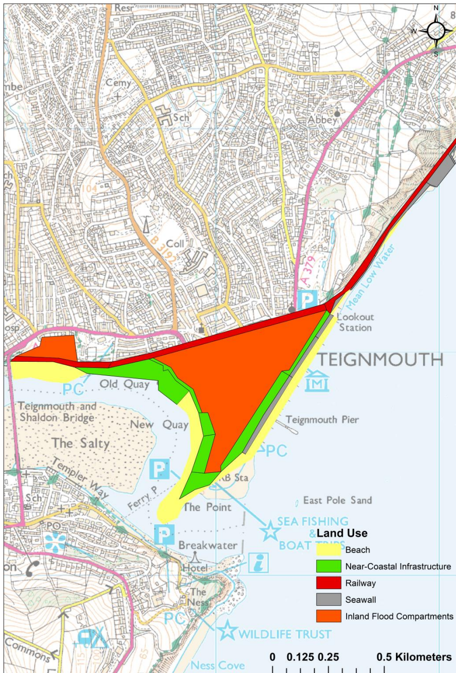
Figure 5: Teignmouth land-use zones and elements for Quasi-2D SPR system diagram (adapted from Narayan, 2014). This map contains Ordnance Survey data © Crown Copyright and database right (2013).
