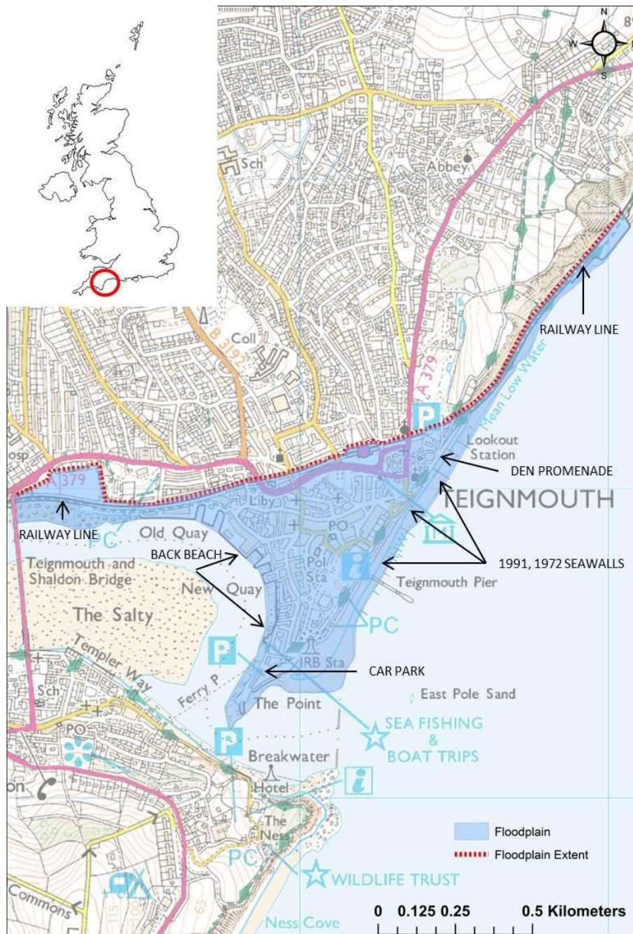
Figure 4: Map of Teignmouth showing floodplain extent and key floodplain elements (Inset: Location of Teignmouth in the UK). This map contains Ordnance Survey data © Crown Copyright and database right (2013).
