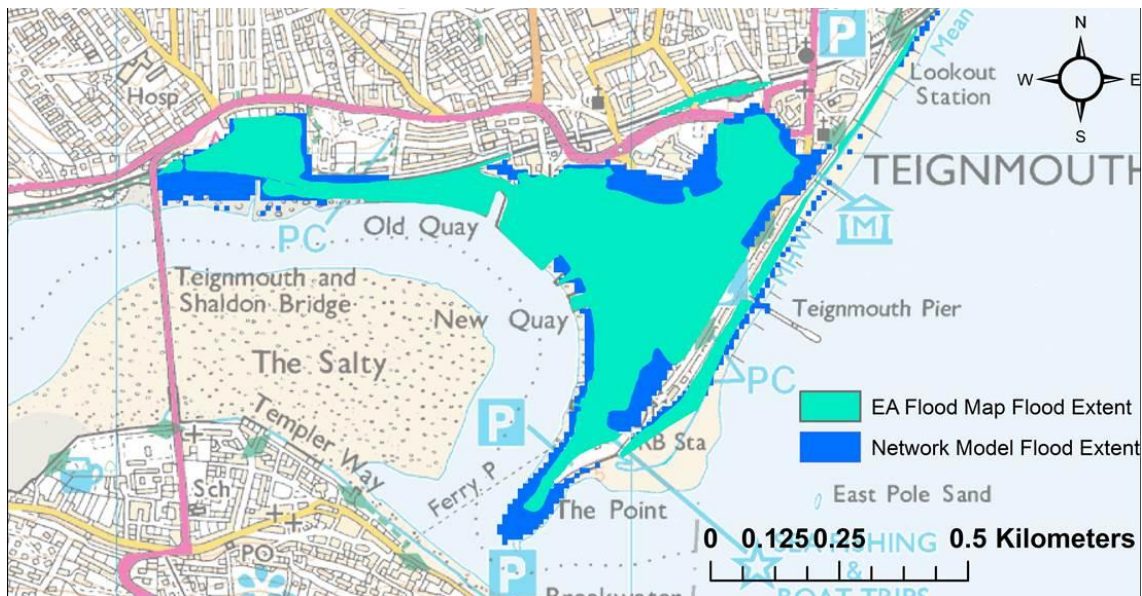
Figure 8: Comparison of Teignmouth network model and EA Indicative flood maps for a 1 in 1000 year ESWL (3.46 m) assuming no defences
