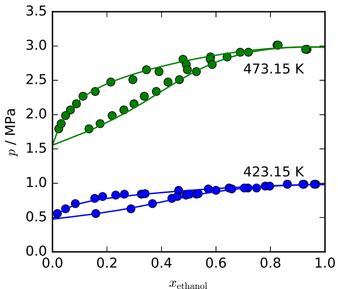
Figure 5: A p - x diagram for the mixture ethanol + water. The experimental data are from Barr-David and Dodge, 47 and the vapor pressure of the pure components are obtained from the ancillary equations of the respective fluid 48
