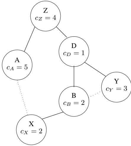
Fig. 2. Tree T(Z) for the example in Figure 1
