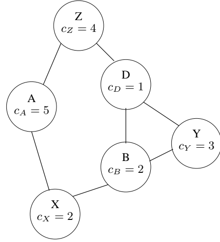
Fig. 1. Example AS graph from Section 4
