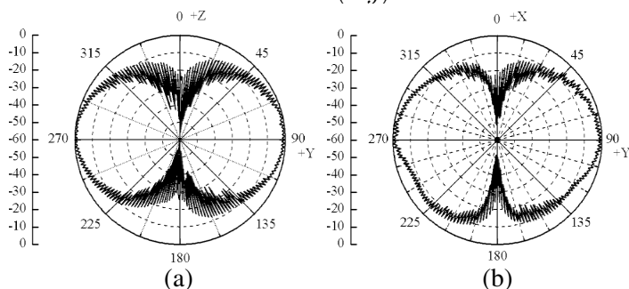
Figure 15. Measured spinning normalised AR patterns of the array at 2.5 GHz. (a) yoz plane. (b) xoy plane.
