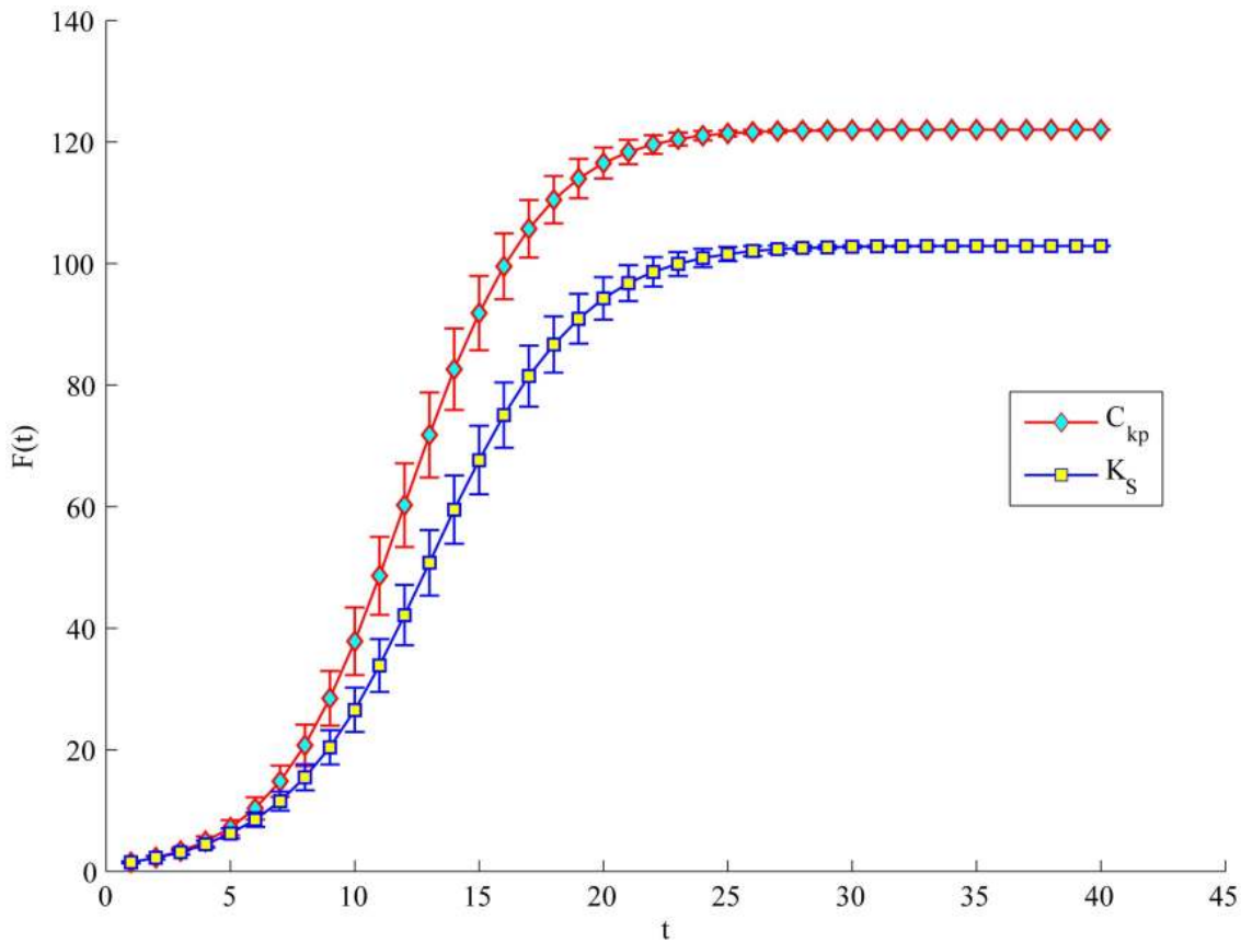
Figure 10. Simulation of top-20 with initial infected to appear by our method with k-shell index (but not both). For each node, F(t) is obtained by averaging over 100 implementations ( \alpha=1.2 ). doi:10.1371/journal.pone.0066732.g010
