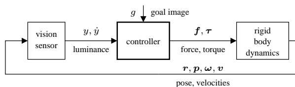
Figure 2. Purely visual pose stabilization. We control in force and torque to stabilize a rigid body based only on the visual input y and \dot{y} , and a memorized goal image g taken at the desired pose. No inertial or velocity sensors are used.
