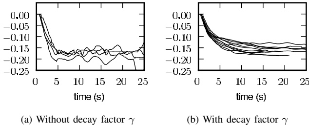
Figure 6. Automatic trim/bias compensation for rudder (rotation about the z -axis) using visual input only, recorded from a number of repeated trials. The compensation term is synthesized by integrating the bilinear velocity estimates \hat{\omega}_{BL} and \hat{v}_{BL} over time. Using a decay factor suppresses the oscillations and gives a stable compensation.
