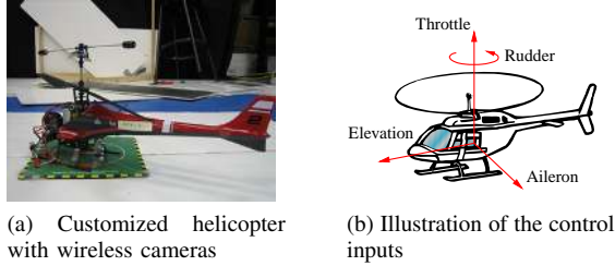
Figure 5. (a) Helicopter used in the experiments, custom-built from E-flite Blade CX2. One wireless camera is encased in the tail boom. (b) Illustration of the control inputs: throttle u_{thr} , rudder u_{rud} , aileron u_{ail} , and elevation u_{ele} .
