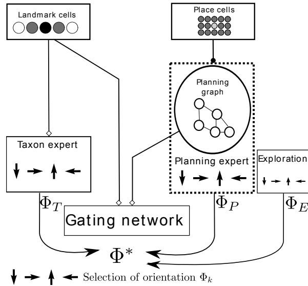
Figure 2. Overview of the (Dollé et al., 2010) model. Different strategies (taxon/topological-map/exploration) are connected to the gating network. Each strategy has a dedicated expert which proposes actions ( \Phi_T for the taxon, \Phi_P for the planing, ...). The gating network decides which of the experts is the winner in the current situation and then the action \Phi^* from this strategy is performed.
