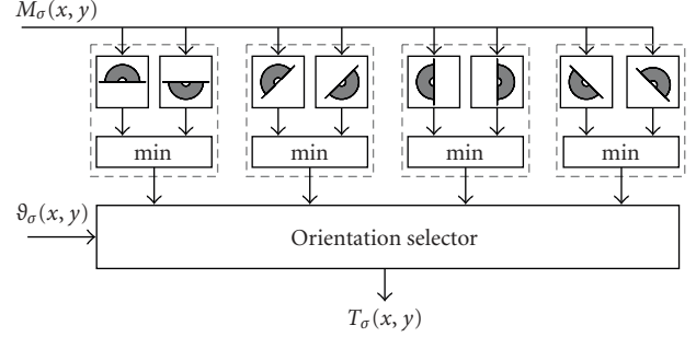
FIGURE 3: Computation scheme of the inhibition term. For each pixel of the image, inhibition terms are computed for a number of different orientations. Then the gradient orientation information is used to select the appropriate value at each pixel.
