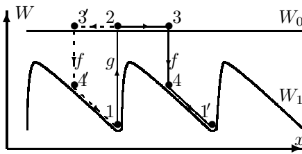
Two-state model for a single motor[6] and Four-phase ATP-cycle
