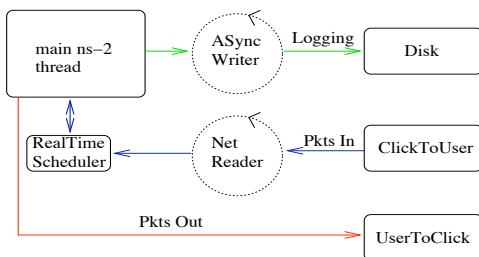
Fig. 2. Relationship between I/O operations and threads in the simulator.
