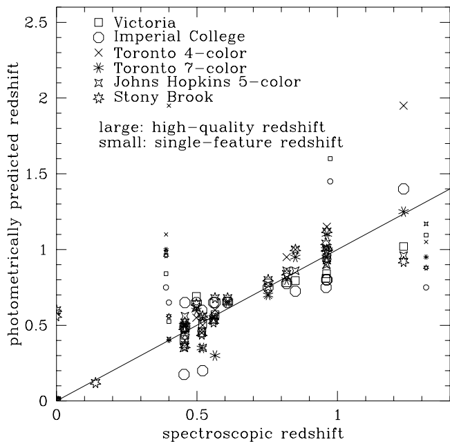
FIG. 1.—Photometric vs. spectroscopic redshifts for the sample. Smaller symbols are used for single-feature spectroscopic redshifts (see text).
