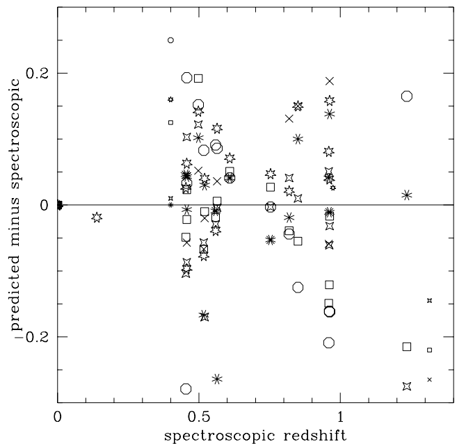
FIG. 2.—Redshift differences, predicted minus spectroscopic, expanded to show only those predictions with differences \Delta z < 0.3 . Symbols are as in Fig. 1.
