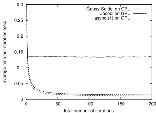
Fig. 8. Average iteration timings of CPU/GPU implementations depending on the total number of iterations, test matrix fv3.
