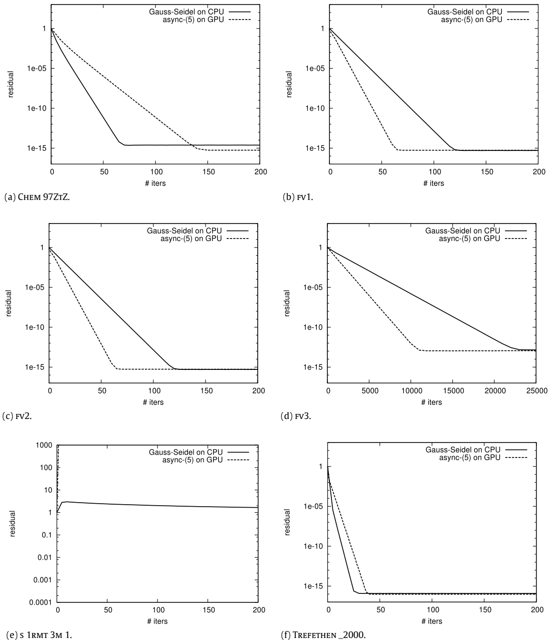
Fig. 7. Convergence rate of block-asynchronous iteration.
