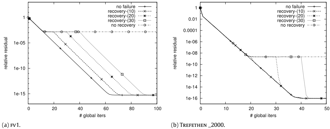
Fig. 10. Convergence of async-(5) for hardware failure. The implementations either recover by reassigning the components to other cores after the recovery time t_r (denoted by recover- t_r ), or generate a solution approximation with a significant residual error.
