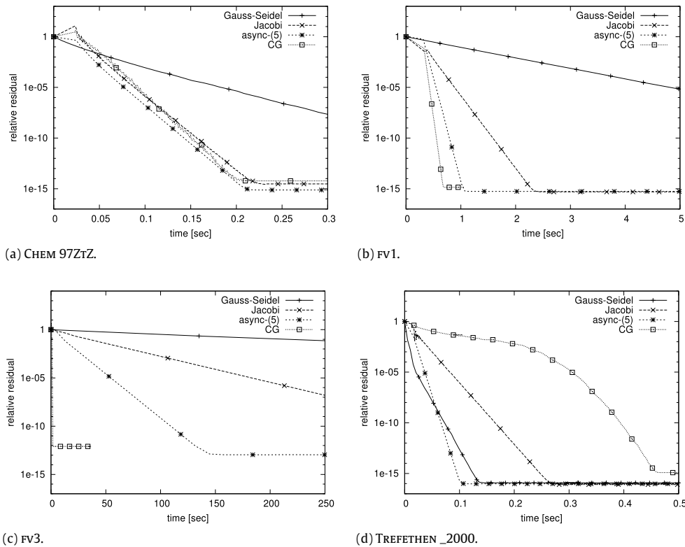
Fig. 9. Relative residual behavior with respect to solver runtime.
