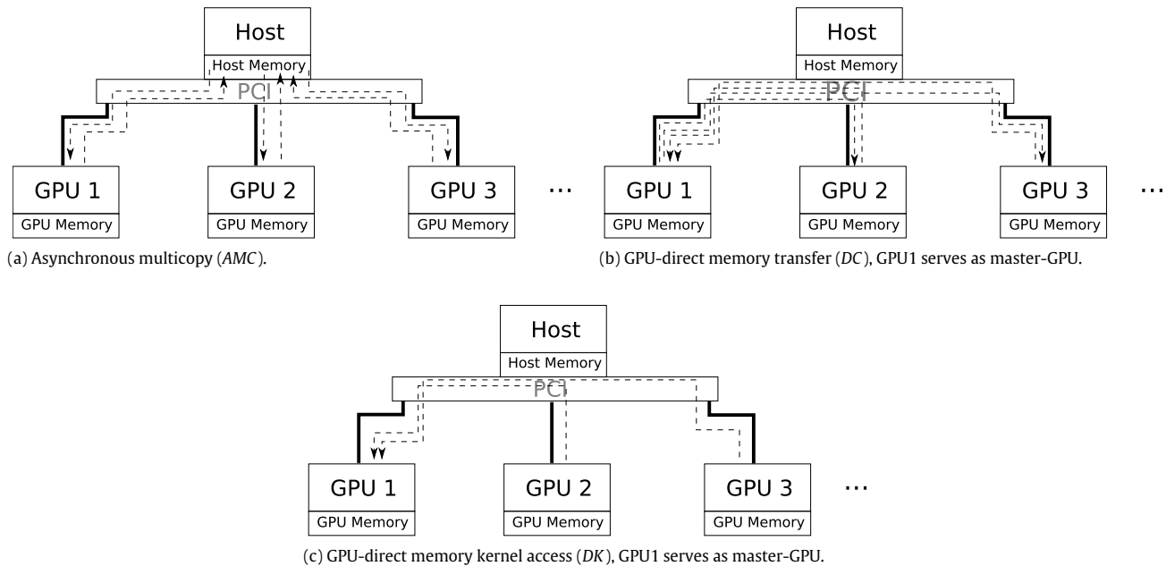
Fig. 4. Visualizing the different multi-GPU memory handling. The dashed lines indicate the explicit data transfers.
